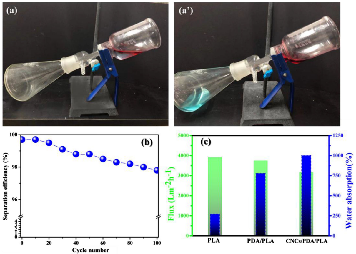
Fig. 6 a(a') Photographs showing the separating process of n-hexane/water mixture by CNCs/PDA/PLA membrane; b Separation efficiency changed with cycle numbers of CNCs/
