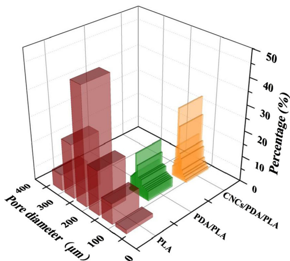
Fig. 4 The pore diameter of pure PLA and CNCs/PDA/PLA nonwoven membranes
