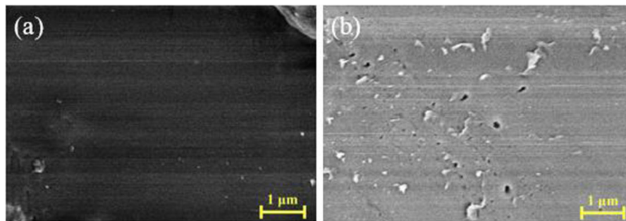
Fig. 8 SEM images of reused membranes: a used for 1 time, b used for 40 times
