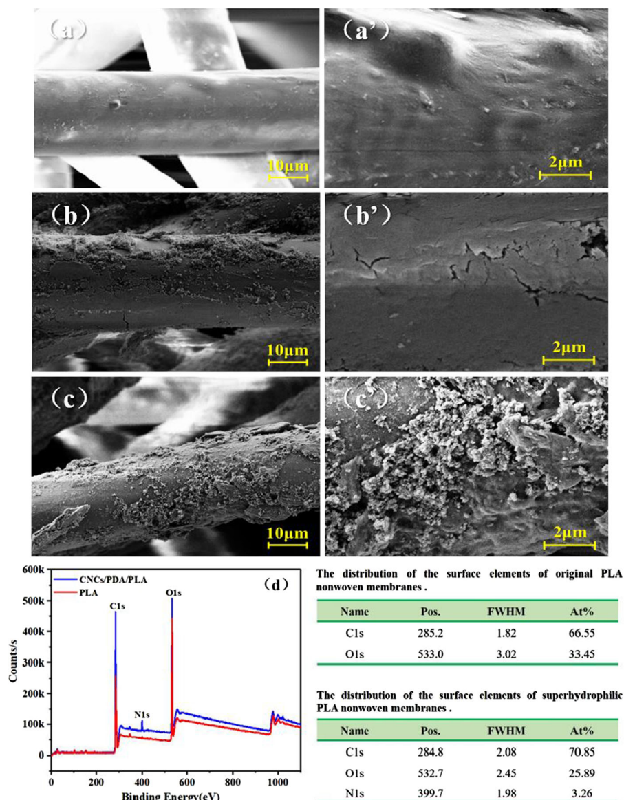
Fig. 3 SEM micrographs of a(a') Pure PLA, b(b') PDA/PLA, c(c') CNCs/PDA/PLA nonwoven membranes. d Element distribution of PLA nonwoven membranes before and after modification by XPS
