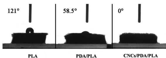
Fig. 5 The water contact angles of pure PLA, PDA/PLA, and CNCs/PDA/PLA nonwoven membranes
