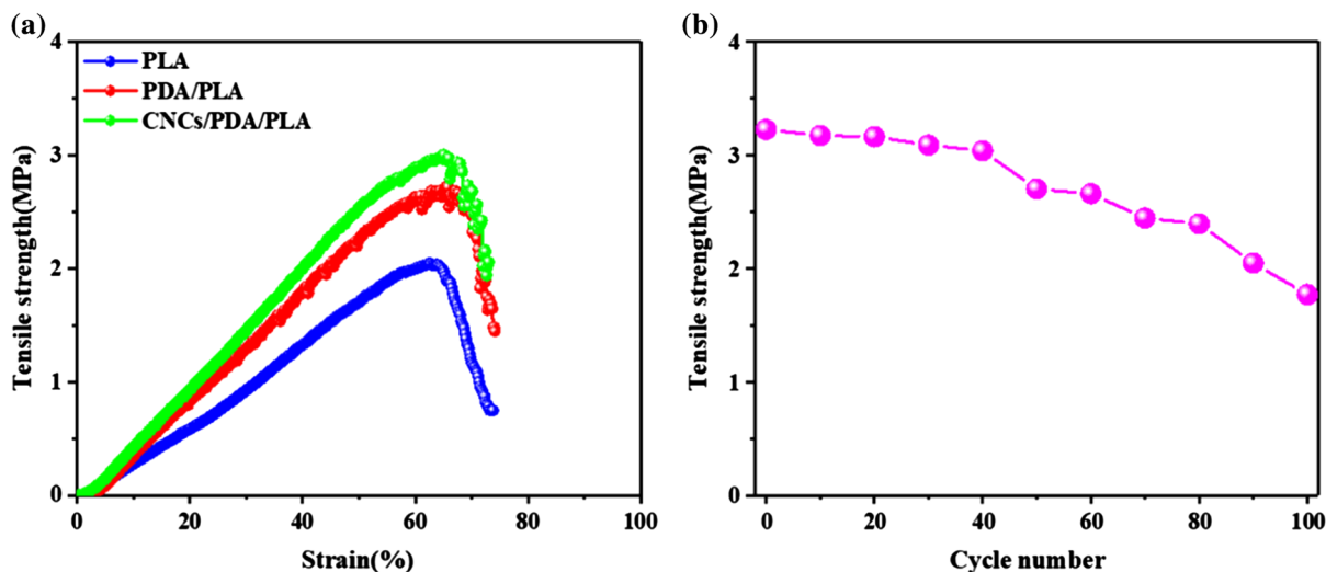
Fig. 7 a Tensile stress–strain curves of pure PLA, PDA/PLA, and CNCs/PDA/PLA nonwoven membranes; b Tensile strength of CNCs/PDA/PLA nonwoven membrane changed with reuse cycle numbers
