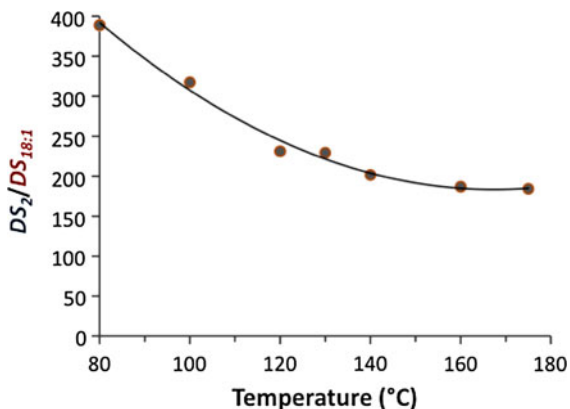
Fig. 4 Influence of the treatment temperature on DS_2/DS_{18:1} (1 h, R = 1.5 )
