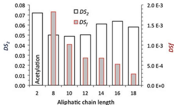
Fig. 6 Influence of the fatty acid aliphatic chain length on DS_2 and DS_f . (140 °C for 1 h, R = 1.5 )
