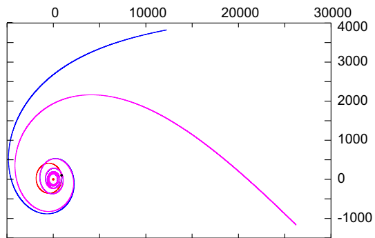
Fig. 7 The orbits for a planet in a planetary system with ICF. The planetary system is obtained from an ordinary planetary system and with elliptical orbits (red) by replacing the ISF forces by ICF and with a strength \beta_3 \approx 1230 \times G . The black circles are the position of the planet at the time where the replacement took place, and the green curve is for \beta_3 = 1228.75 and the blue curve is for \beta_3 = 1228.5
