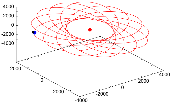
Fig. 4 A planet which after 13 orbits almost returns to its start position. The start position at t = 2.5 \times 10^6 is shown with a big blue sphere, and the position at t = 2.5051975 \times 10^6 after 13 orbits by a smaller black sphere. The next figure shows several orbits of the planet together with the orbits of the outermost planet
