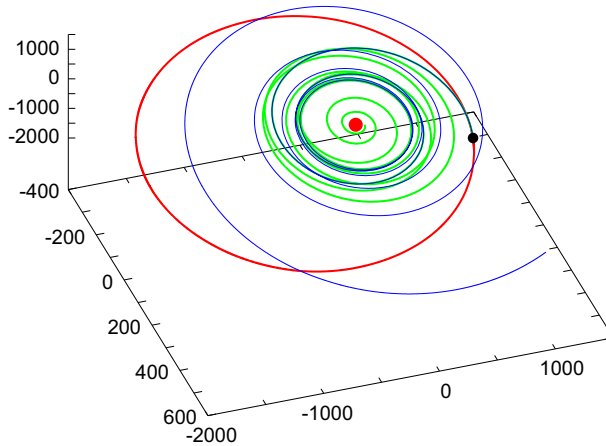
Fig. 7 The orbits for a planet in a planetary system with ICF. The planetary system is obtained from an ordinary planetary system and with elliptical orbits (red) by replacing the ISF forces by ICF and with a strength \beta_3 \approx 1230 \times G . The black circles are the position of the planet at the time where the replacement took place, and the green curve is for \beta_3 = 1228.75 and the blue curve is for \beta_3 = 1228.5
