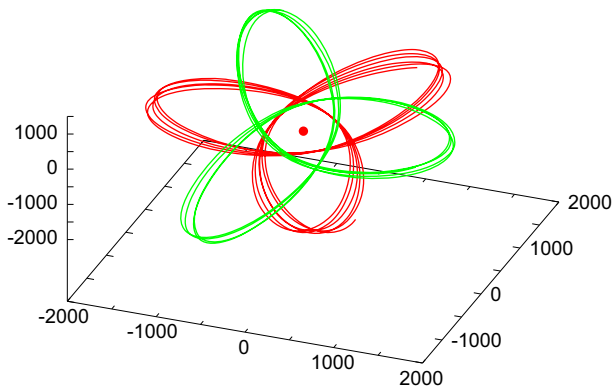
Fig. 2 The simultaneous orbits with bows for two other planets in the planetary system. The orbits are obtained for one million discrete time steps in the time interval t \in [2.5 \times 10^6, 2.5025 \times 10^6]
