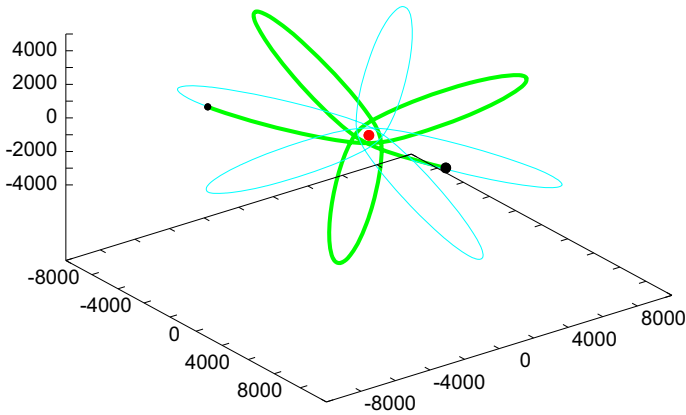
Fig. 3 Bows in a loop with green and light blue for the outermost planet. The start position at t = 2.5 \times 10^6 is marked with a big black sphere, and the first three bows are marked with green. The position at t = 2.5025 \times 10^6 after the first three bows is shown by a smaller black sphere, and the succeeding five bows are marked with light blue. Several consecutive loops of the planet are shown in Figure 5
