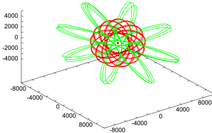
Fig. 5 The outermost planet (green) together with the planet from Fig. 4 (red) with its orbits in bands. The outermost planet changes its major orbit axis with \approx \pi/4 at every part of the Sun. The central Sun is marked with red
