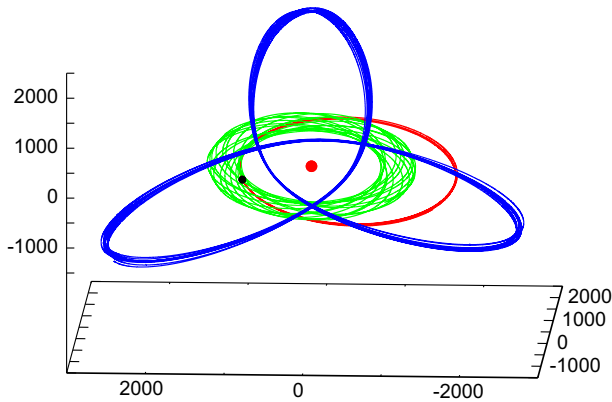
Fig. 6 The red elliptical orbits are for a planet with Newtonian ISF forces and the green orbits are after the forces at the position marked with a black sphere replaced with IF forces and with \beta_1=0.00105 by which the planet in a short time follows the elliptical path before the revolving behaviour. The orbit (blue) of a planet at a mean distance slightly bigger than the planet shown by red changed spontaneously its elliptical orbit to the bows also shown in the previous figures
