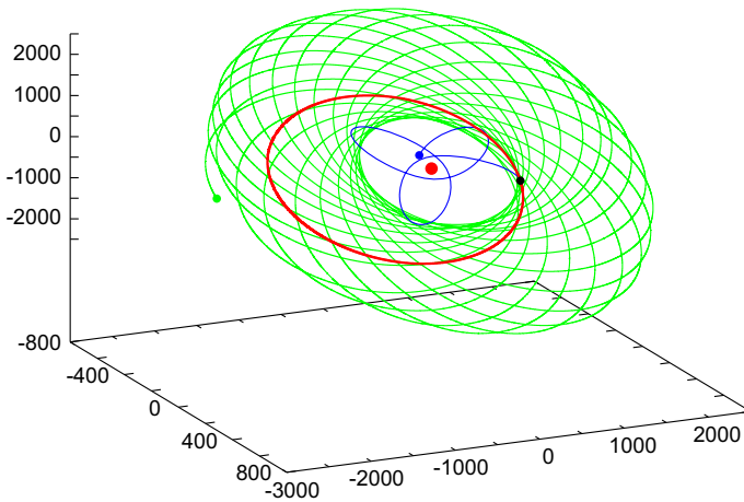
Fig. 9 The planet also shown in Fig. 7 in red, but now with IF or ICF included in the ISF attraction. The orbit in red is with pure ISF; the orbit in green is with ICF: \alpha_3/r^3 = -100/r^3 included from the position marked by a black sphere, and the orbit in blue is with the IF: \alpha_1/r = 0.01/r included. The planet with ISF + ICF in green has revolved \approx 23 – 24 times before the principal axis in the elliptical orbit has changed 2\pi
