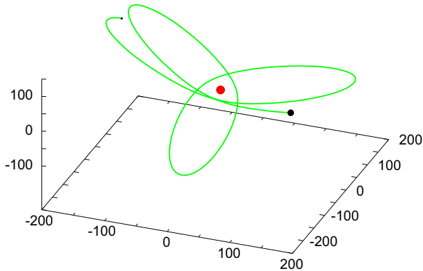
Fig. 1 A loop of the innermost planet from a position at time t = 2.5 \times 10^6 , marked by a big black sphere to a position at t = 2.5007325 \times 10^6 (293000 discrete time steps), marked by a small black sphere. The position of the “Sun” is with an enlarged red sphere. Some simultaneous loops of two other planets in the planetary system are shown in the next figure
