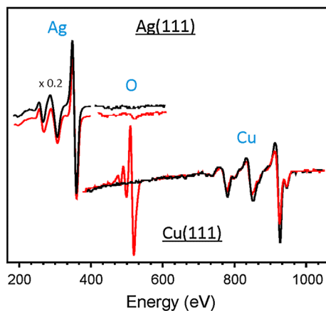
Fig. 5 Auger spectra of Ag(111) and Cu(111) surfaces before ( black lines ) and after ( red lines ) the CO oxidation reaction. Formation of a CuO x overlayer is clearly observed on Cu(111), whereas the Ag(111) surface remains metallic
