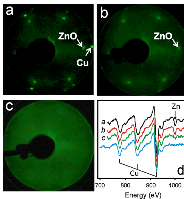
Fig. 6 LEED (a–c) and corresponding AES (d) results for the 0.8 ML ZnO/Cu(111) film: as prepared (a), after exposure to the reaction mixture at 300 K for 10 min (b), and 450 K for 1 min (c). The bottom ( blue ) spectrum in (d) was obtained for the spent catalyst after 30 min of the reaction at 450 K. Cu and Zn Auger transitions are indicated
