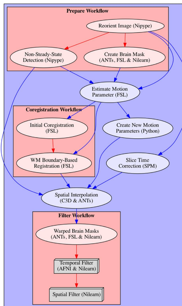
Fig. 2 Depiction of fMRIfloWS' functional preprocessing pipeline. Arrows indicate dependency between the different processing steps and data flow. Name of each node describes functionality, with the corresponding software dependency mentioned in brackets. Steps that can be grouped into specific sections are contained within a red box to facilitate understanding of the pipeline. Color of arrows indicated if connection stays within a section (red) or not (blue). Nodes depicted as gray boxes indicate that they can be run multiple times with iterating input values, i.e. performing a spatial smoothing with an FWHM value of 4 and 8 mm (Color figure online)
