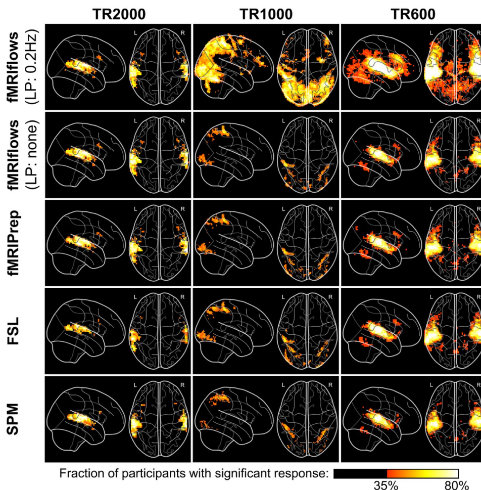
Fig. 11 Depiction of binarized 1st-level activation count maps, thresholded at p < 0.001 , after multiple functional preprocessing approaches. Preprocessing was done with fMRIflows (with and without a temporal low-pass filter at 0.2 Hz), fMRIPrep, FSL and SPM (from top to bottom) separated for the TR2000 (left), TR1000 (middle) and TR600 (right) dataset. Activation count maps were normalized to the ICBM 2009c brain template. Color code represents the fraction of participants that show significant activation above a p -value threshold at 0.001 and corrected for false positive rate (FPR) (Color figure online)
