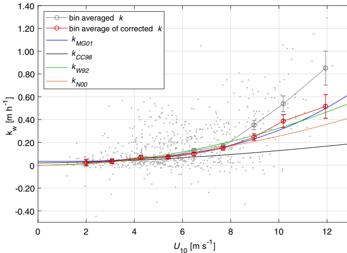
Fig. 10 Wind speed versus the gas transfer velocity, k , determined from the fluxes during open-water situations. The fits represent the 1 \text{ m s}^{-1} bin-averaged data (grey) and the bin-averages of the k determined from the corrected flux (red). The error bars give the standard error. Also, commonly used wind speed based parametrizations by McGillis et al. (2001) ( k_{MG01} ), Cole and Caraco (1998) ( k_{CC98} ), Wanninkhof (1992) ( k_{W92} ), and Nightingale et al. (2000) ( k_{N00} ) are shown
