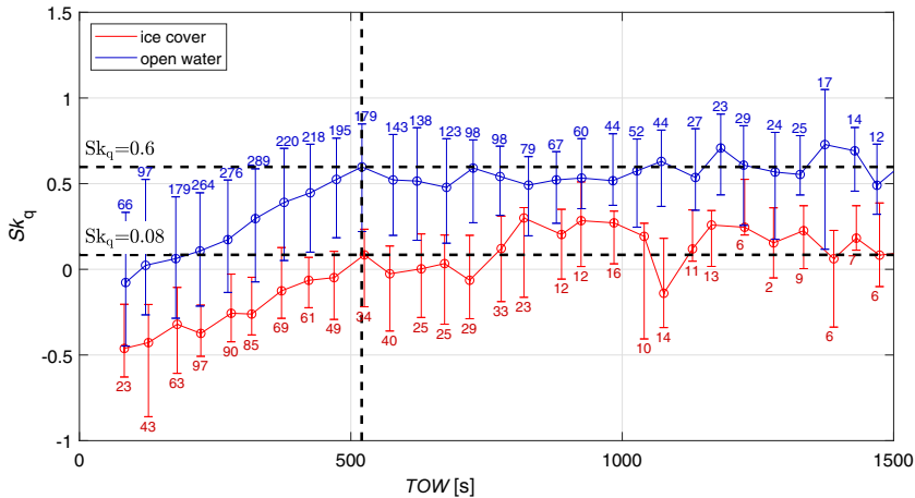
Fig. 6 Bin-averaged time over water ( TOW ) versus humidity skewness ( Sk_q ) for ice-covered (red) and open-water conditions (blue). The error bars give the 25 and 75 percentiles. The numbers at the error bars indicate the amount of samples in each bin. The horizontal and vertical dashed lines give the Sk_q and TOW at which the relations level off. These thresholds are indicated in Fig. 4 by the vertical dashed lines
