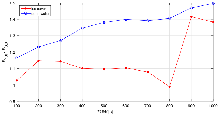
Fig. 7 Time over water ( TOW ) versus the ratio of the first to third quadrant for a hole size of zero ( S_{1,0}/S_{3,0} ) for ice-covered (red) and open-water conditions (blue)
