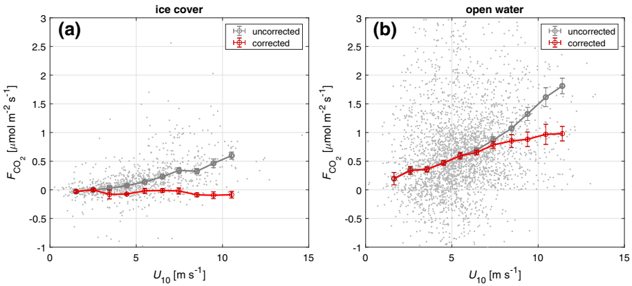
Fig. 9 Wind speed versus F_{CO_2} for all data of a ice-covered and b open-water situations. The fits represent the 1 \text{ m s}^{-1} bin-averaged data (gray) and the bin-averages of the corrected flux based on the fits in Fig. 8 (red). The error bars give the standard error
