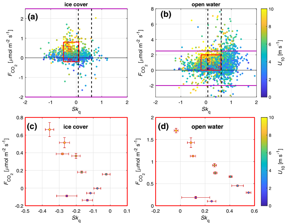
Fig. 4 Skewness versus CO 2 flux with the colour coding representing U_{10} for a ice-covered and b open-water conditions. The range of F_{\text{CO}_2} on the y-axis is different for a , b . The range of the ice-covered fluxes is denoted by horizontal purple lines in b . The vertical dashed lines show the Sk_q -thresholds for non-locally and locally dominated processes as defined in Fig. 6. The red circles in a , b show the data binned according to the wind speed level. This binned data is also shown in the same set-up but zoomed-in in c for ice-covered, and d open-water conditions. The zoomed-in windows are highlighted as red squares in a , b respectively. The error bars show the standard error
