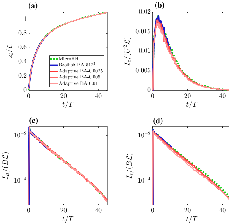
Fig. 8 Time series of the domain integrated quantities, a boundary-layer height ( z_i ), b kinetic energy ( I_e ), c buoyancy flux ( I_B ) and d dissipation rate ( I_\epsilon ) according to Eq. 11. The results are obtained with both Basilisk and MicroHH solvers using fixed grids and Basilisk using the adaptive mesh refinement algorithm. Note that plots c , d use a logarithmic scale
