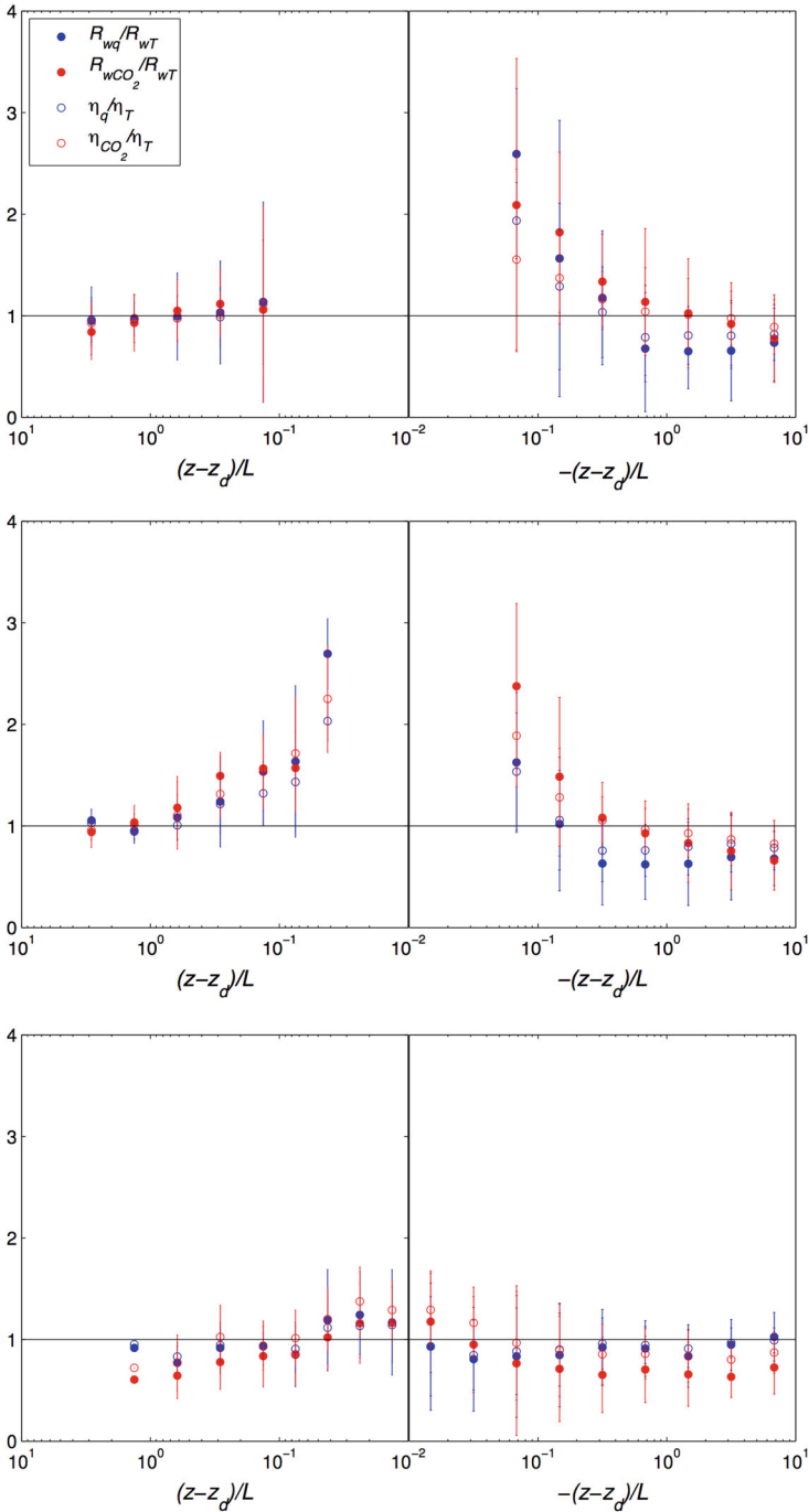
Fig. 9 Ratios of transport efficiencies of water vapour and CO 2 to the transport efficacy of heat under stable (left panels) and unstable (right panels) conditions at 47 m (bottom panel), 140 m (middle panel) and 280 m (top panel). The vertical error bars denote the standard deviation within each bin
