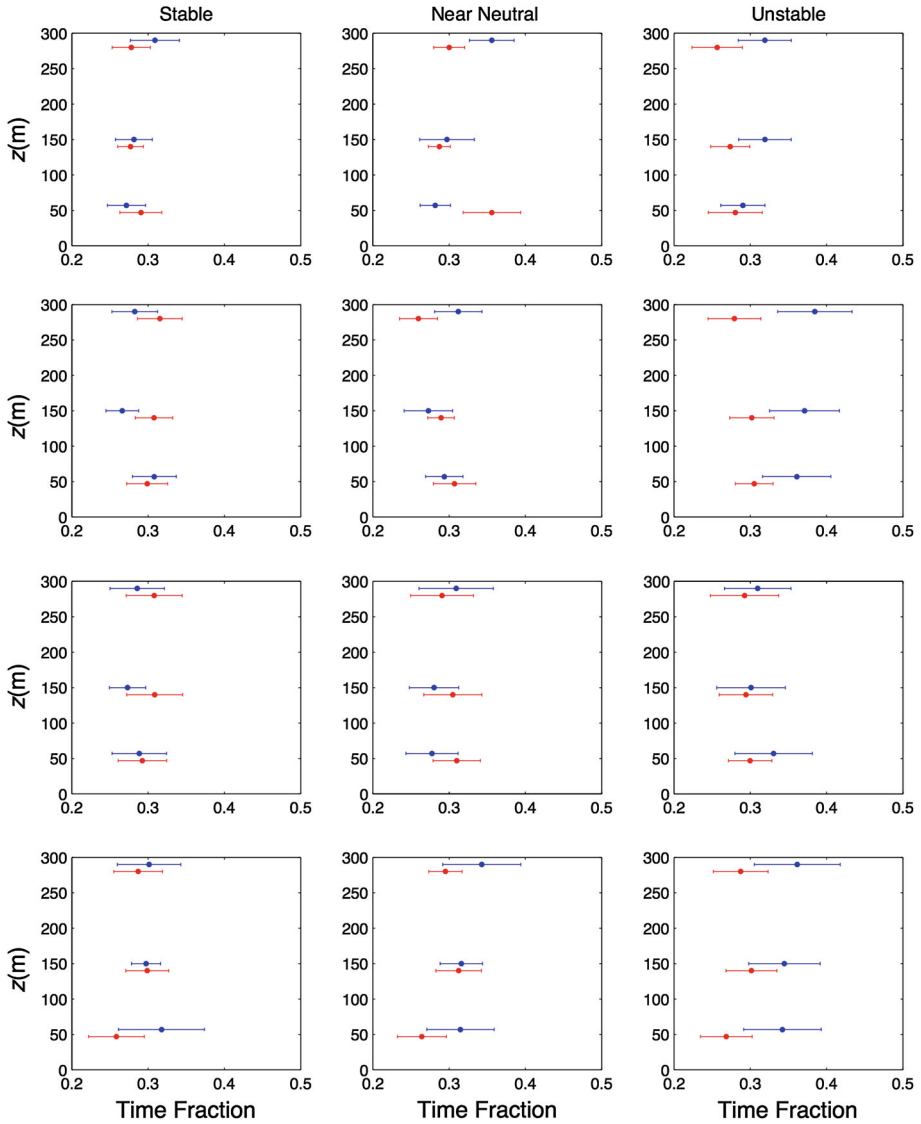
Fig. 5 Time fractions of ejections ( red dots ) and sweeps ( blue dots ) for momentum flux, sensible heat flux, latent heat flux and CO 2 flux (from top to bottom ) under stable, near-neutral, and unstable conditions (from left to right ) at three levels (47, 140, and 280 m). The blue dots are shifted up by 10 m in order to compare with the red dots
