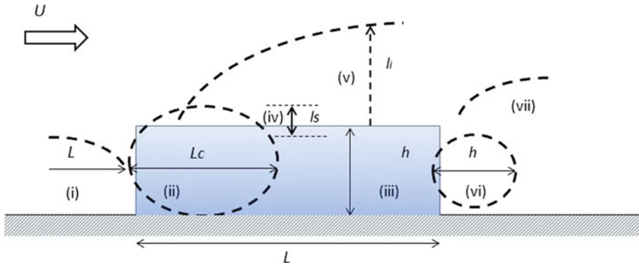
Fig. 1 Schematic showing different zones of adjustment to the canopy transition according to Belcher et al. (2003). (i) Impact region; (ii) adjustment region; (iii) canopy interior; (iv) canopy shear layer; (v) roughness-change region; (vi) exit region; (vii) far wake. The quantities h , L , L_c , l_s denote canopy height, length of canopy stretch, adjustment length scale and height of the canopy shear layer respectively
