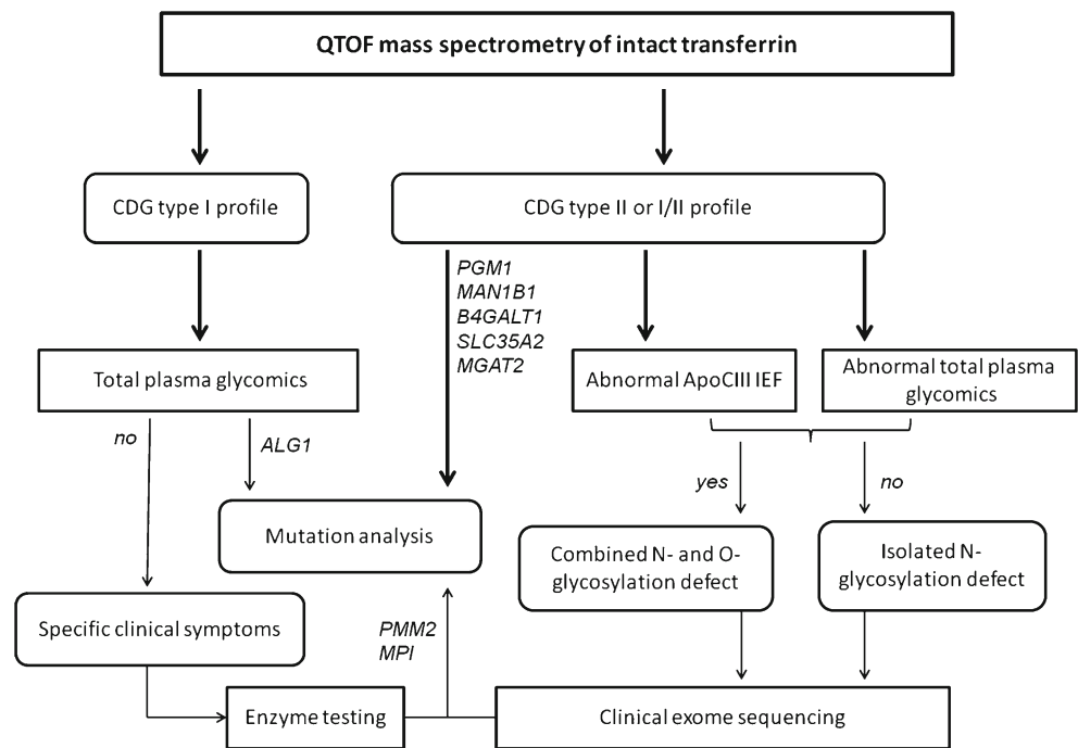
Fig. 3 Clinical diagnostic flowchart for CDG. The combination of mass spectrometry with clinical exome sequencing and clinical phenotyping allows facile identification of the majority of known CDG-I and CDG-II subtypes in a diagnostic setting. The gene defects mentioned here are examples of characteristic diagnostic glycomics profiles in our laboratory. Please refer to Jaeken and Peanne (2017) and Peanne et al (2017) for clinical symptoms in CDG
