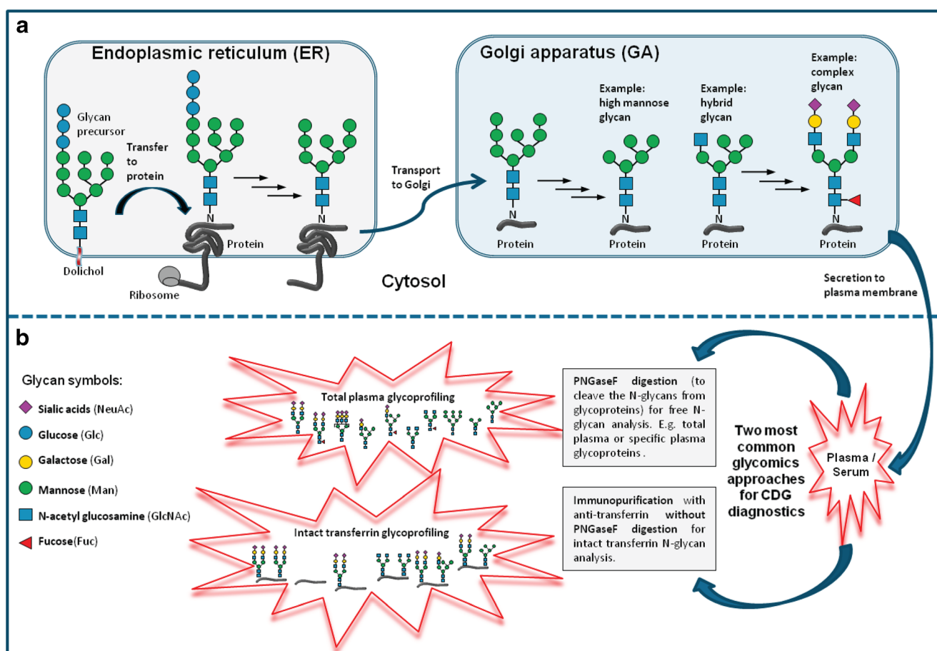
Fig. 1 Schematic representation of the process of protein N-glycosylation, the different types of N-glycans (a) and their analysis by mass spectrometry in CDG (b) (a) The process of N-glycosylation is started when a glycan precursor is assembled by sequential addition of monosaccharides onto the lipid anchor dolichol in the membrane of the ER. The glycan precursor containing 14 monosaccharides (Glc 3 -Man 9 -GlcNAc 2 ) is then transferred en bloc to a specific asparagine residue (N) within the consensus sequence N-X-S/T (X = any amino acid except proline, S = serine, T = threonine) in the nascent peptide chain of a protein (e.g., transferrin) being synthesized by a ribosome. After several glucose trimming by ER glucosidases, the glycoprotein is transported to the GA, where the glycans are modified in multiple steps through the action of
