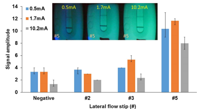
Fig. 7 Experimental results detected by the handheld optical reader with different driving currents. Inset shows recovered photographs of standard lateral flow strips taken by the handheld optical reader
