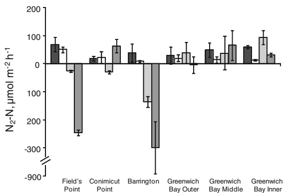
Fig. 2 Spatial distribution of mean net N_2 -N fluxes for stations 1–6. N_2 -N fluxes are averaged by temperature: 6°C (dark bar), 14°C (open bar), 17°C (light grey bar), 22°C (dark grey bar). Temperatures are 1°C
