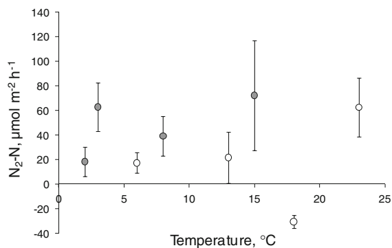
Fig. 4 N 2 -N fluxes (mean ± SD) as a function of temperature measured in 1979 by Seitzinger (1984) (shaded circle) and those of this study (open circle) for Conimicut Point
