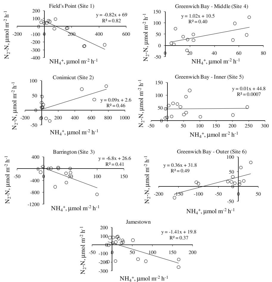
Fig. 3 Sediment net N_2-N fluxes as a function of sediment ammonium fluxes for seven sites in Narragansett Bay. Significant correlations are observed for all of the sites except Greenwich Bay Inner (Site 5) (Site 5)
