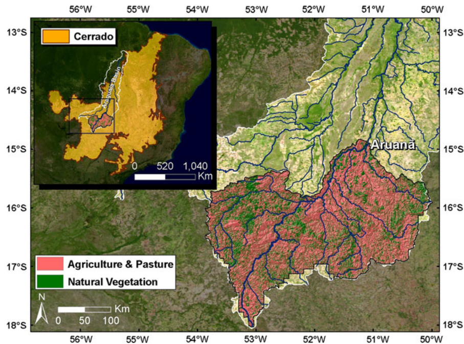
Fig. 1 Main figure: The 82,632 km 2 Araguaia River watershed upstream of Aruanã showing classification of remnant Cerrado and altered lands. About 54% of the basin vegetation was altered as of 2002. Inset: Eastern South
