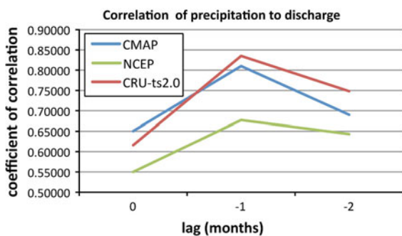
Fig. 2 Lagged Pearson product moment coefficient of correlation ( r ) between the 228 monthly mean precipitation and discharge values for the period 1980–1998. Values are spatially averaged over the 82,632 km 2 Aruanã watershed for the CRU-ts2.0, NCEP, and CMAP datasets. All data show best linear relationship of precipitation to discharge when the month of peak precipitation lags the discharge peak by 1-month (−1)
