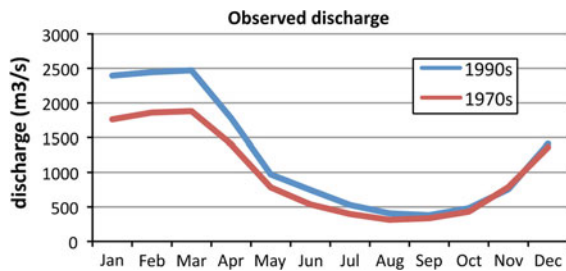
Fig. 4 Decadal mean monthly observed discharge in \text{m}^3/\text{s} at Aruanã for the 1970s and 1990s
