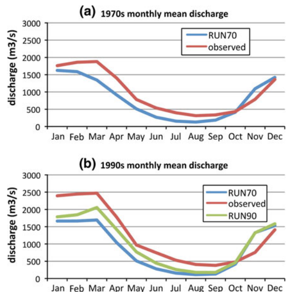
Fig. 5 Decadal mean monthly discharge in \text{m}^3/\text{s} at the Aruanã station for the observations, RUN70 simulation, and RUN90 simulation at Aruanã. a 1970s decadal mean and b 1990s decadal mean. RUN70 has the transient climate of the period 1970–2000 with land cover fixed to the 1970s mean distribution of about 28% deforested. RUN90 has the transient climate of the period with the land cover fixed to the 1990s mean distribution of about 56% deforested. Differences between RUN70 and RUN90 in the 1990s ( b ) are attributable solely to the land cover differences
