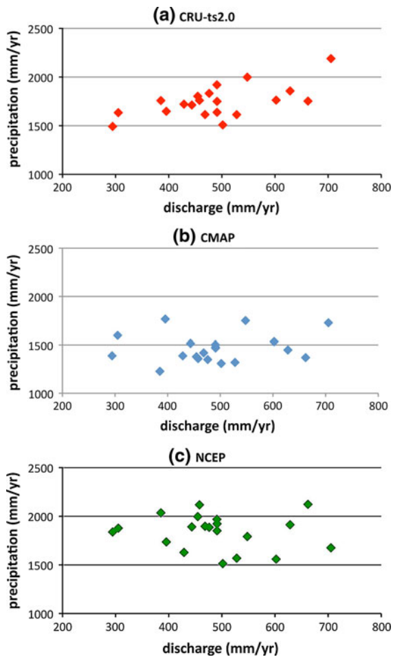
Fig. 3 Scatter diagrams of annual mean precipitation averaged for the Aruanã watershed versus observed discharge at the Aruanã gauge for the period 1980–1998 for a CRU-ts2.0, b CMAP, and c NCEP precipitation products. The sample size is 19 for each series
