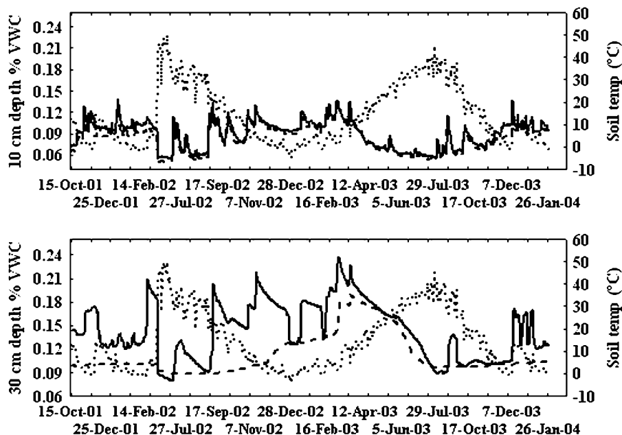
Figure 3. TDR soil-moisture and temperature data for soils at the Squaw Flat site. The top graph shows percent soil moisture (VWC) and temperature in ^{\circ}\text{C} at 10 cm below the surface. The bottom graph shows percent soil moisture and temperature at 30 cm below the surface. Both graphs have the same line symbology; (— VWC 82% sand), (- - - VWC 48% sand), (..... soil temperature). Data from March 2002 through June 2002 are not shown.
