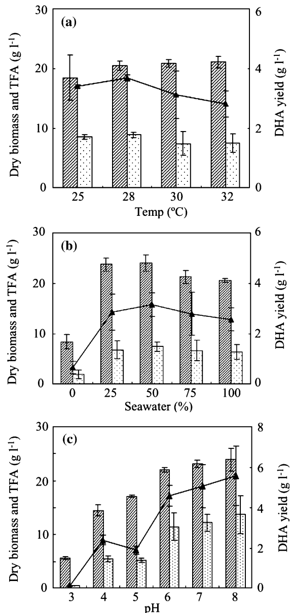
Fig. 2. Effects of growth temperature (a), seawater concentration (b), and pH on biomass, TFA, and DHA yields of strain 12B. Cells were grown at 28 °C (b and c) for 2 days with shaking at 180 rpm in F medium consisting of 5% (w/v) glucose (a), 1% (w/v) yeast extract, 1% (w/v) peptone, and 50% (v/v) seawater (a and c). In (a) and (b) pH was not adjusted. In (b) and (c) glucose concentration was 8%. Hatched and dotted bars represent dry biomass and TFA, respectively. Solid line shows DHA yield. Values represent the averages of triplicate determinations.
