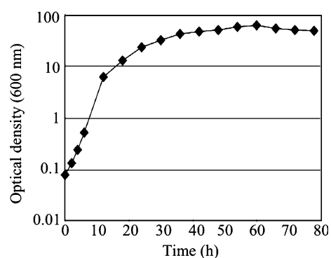
Fig. 3. Growth profile of strain 12B under optimal conditions.
