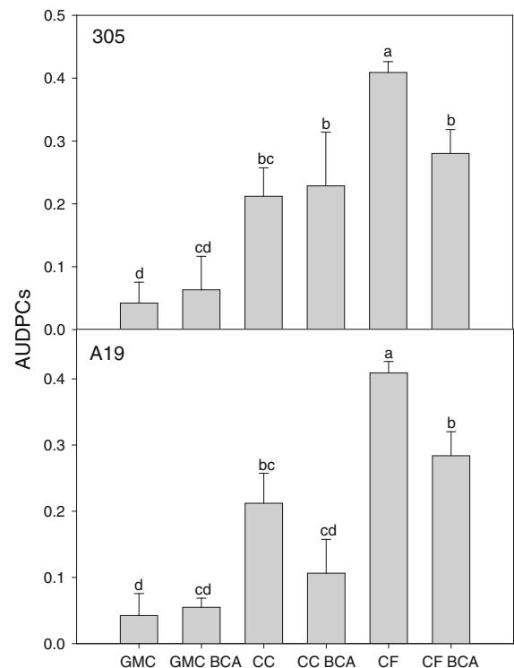
Fig. 1 Standardized areas under disease progress curve (AUDPCs) for tomato plants cultured in three growing media (GMC grape marc compost, CC cork compost, CF coir fiber) inoculated or not with isolate 305 or A19. All these treatments were artificially infested with F. oxysporum f. sp. lycopersici race 2 (FN2). Bars with the same letters were not significantly different ( P \leq 0.05 ) according to LSD test ( F_{5,18} = 11.10 and 14.16 and P = 0.0001 and <0.0001 for AUDPCs in 305 and A19 respectively). Analysis of variance was performed with arcsine ( \sqrt{x} ) transformed data. Error bars represent SE ( n = 6 )
