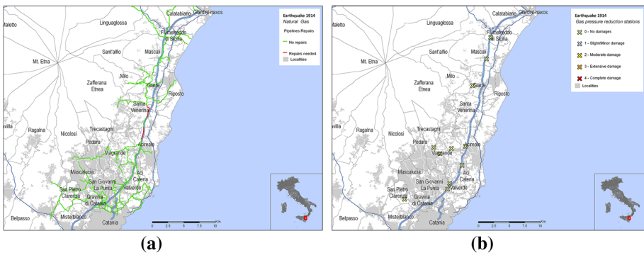
Fig. 9 Damage to the natural gas system in the study area. a Pipelines. b Pressure reduction and measurement stations
