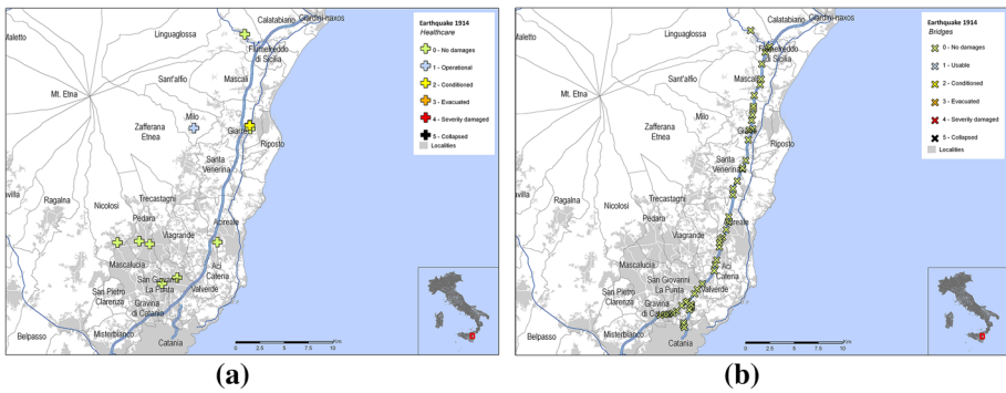
Fig. 8 Damage to healthcare buildings a and motorway bridges b in the study area
