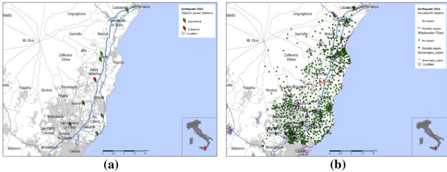
Fig. 10 Damage to the electricity power stations a and water and wastewater systems b in the study area
