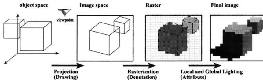
Figure 5. The traditional computer graphics pipeline.
