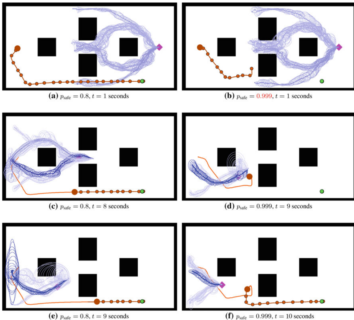
Fig. 12 Representative screenshots of the RR-GP and CC-RRT algorithms as the host vehicle approaches the first waypoint in the complex scenario, for two different values of p_{\text{safe}}
