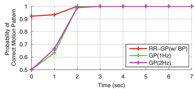
Fig. 5 Average probability (over 90 trajectories) of the correct motion pattern for RR-GP (w/ BP), Sparse-GP (1 Hz), and Dense-GP (2 Hz) algorithms as function of time. For example, the values at t = 1 s represent the probability of the correct motion patterns after the target vehicle has actually moved for 1 s on its path
