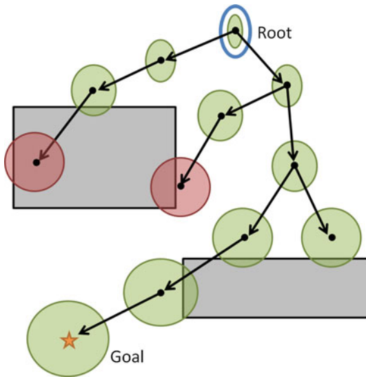
Fig. 8 Diagram of the chance constrained RRT algorithm. Given an initial state distribution at the tree root (blue) and constraints (gray), the algorithm grows a tree of state distributions to find a probabilistically feasible path to the goal (yellow star). The uncertainty in the state at each node is represented as an uncertainty ellipse. If the probability of collision is too high, the node is discarded (red); otherwise the node is kept (green) and may be used to grow future trajectories (Color figure online)
