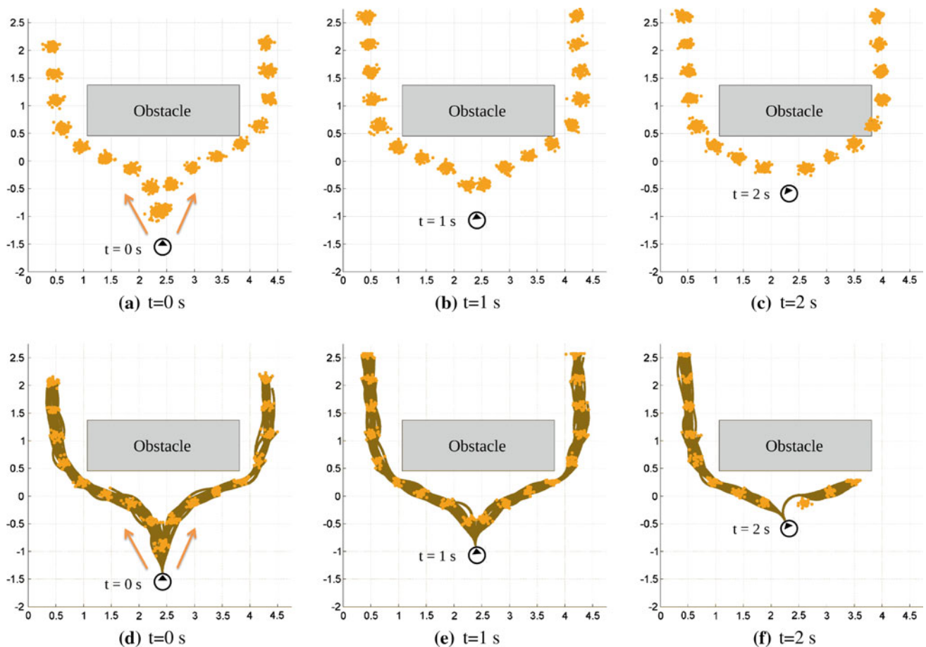
Fig. 3 Snapshots of the GP samples ( top row ) and Algorithm 2 output ( bottom row ) on a test trajectory
