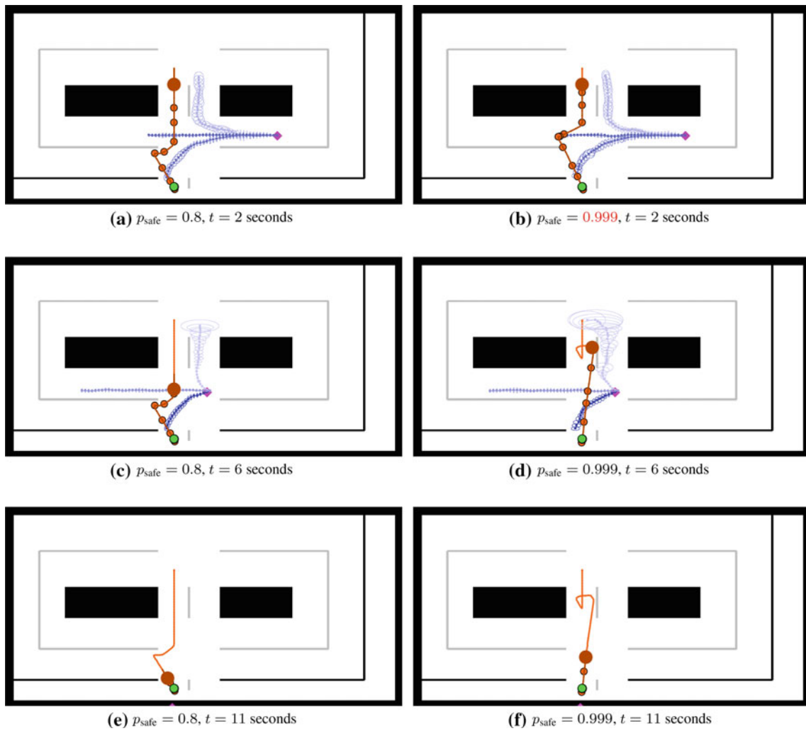
Fig. 10 Representative screenshots of the RR-GP and CC-RRT algorithms during trial #25 of the intersection scenario, for two different values of p_{\text{safe}} . The host vehicle’s path history and current path are in orange. The objective of the host vehicle (large orange circle) is to reach the goal position (green circle) while avoiding all static obstacles (black) and the dynamic target vehicle (magenta diamond). The blue
