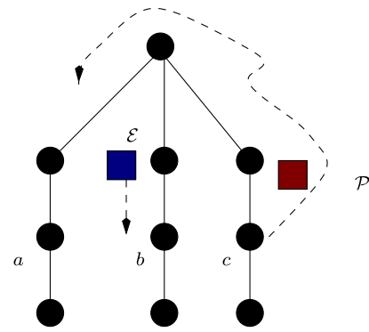
Fig. 2 Both players have 1-visibility. On this graph, the pursuer \mathcal{P} can not capture the evader \mathcal{E} using a deterministic strategy. However, a randomized capture strategy exists (from Isler et al. 2006)
