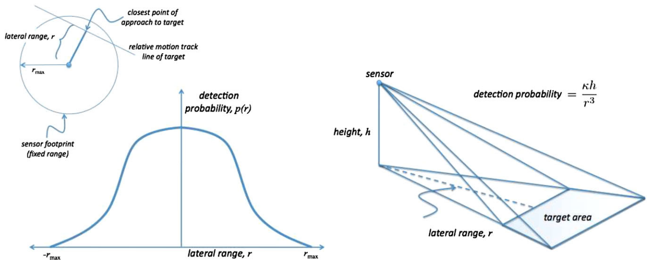
Fig. 5 Illustration of mathematical models for sensor detection characteristics. Left : the lateral range curve for a range-dependent sensor such as sonar. Right : an inverse cube model for visual (aerial) sightings
