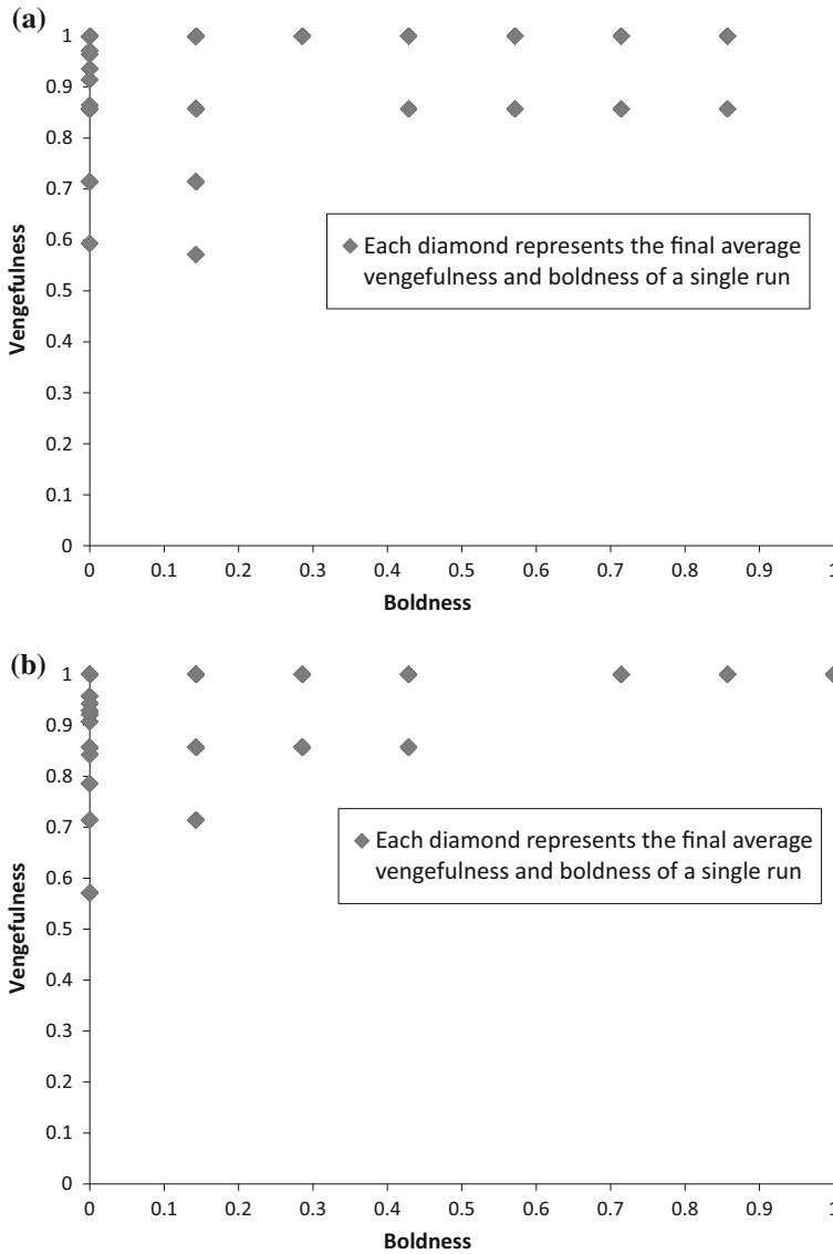
Fig. 10 No-mutation metanorms game. a 100 generations without mutation b 1,000,000 generations without mutation
