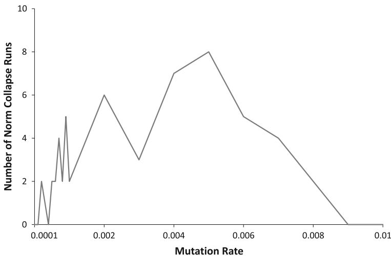
Fig. 8 Metanorms game: 1,000,000 generations; 0.0001–0.01 mutation rate
