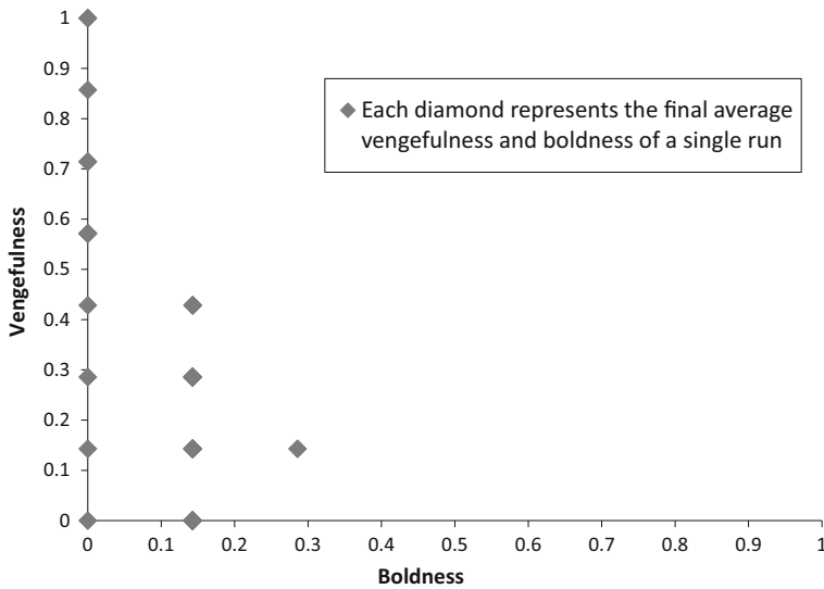
Fig. 9 No-mutation norms game: 1,000,000 generations and 1000 runs
