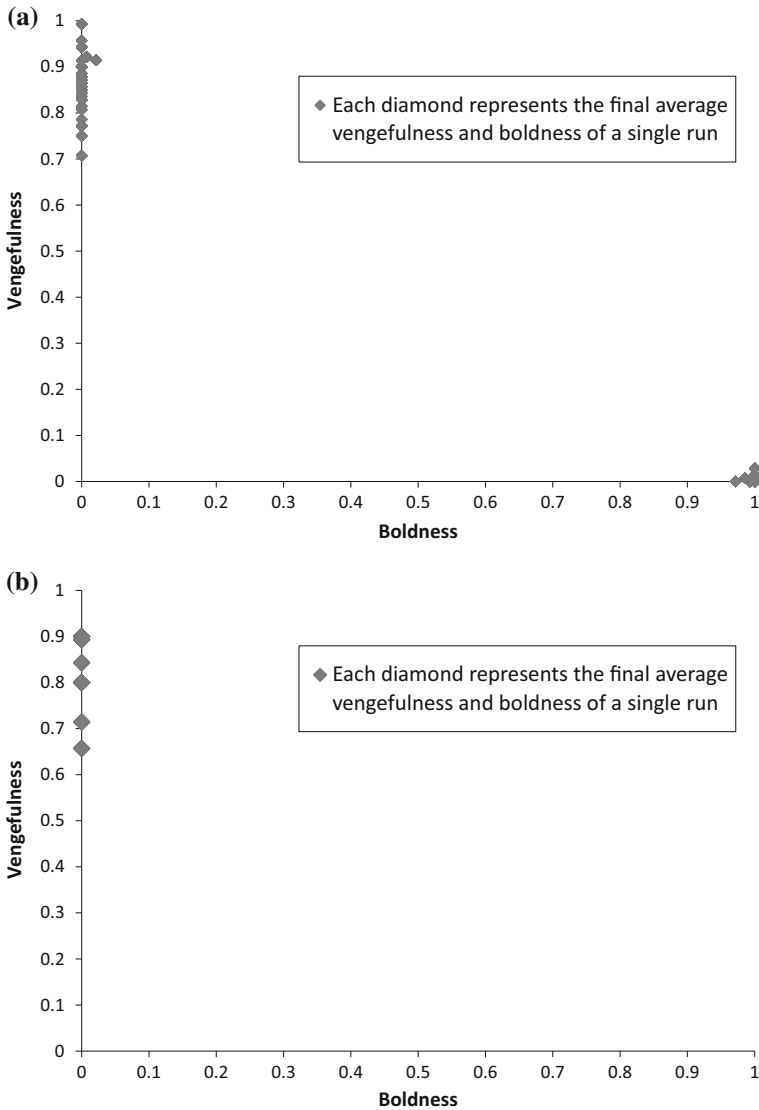
Fig. 7 Metanorms game with different mutation rates. a 1,000,000 generations and 0.001. mutation rate. b 1,000,000 generations and 0.0001 mutation rate
