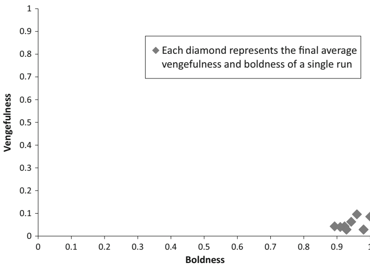
Fig. 5 Norms game for 1,000,000 generations
