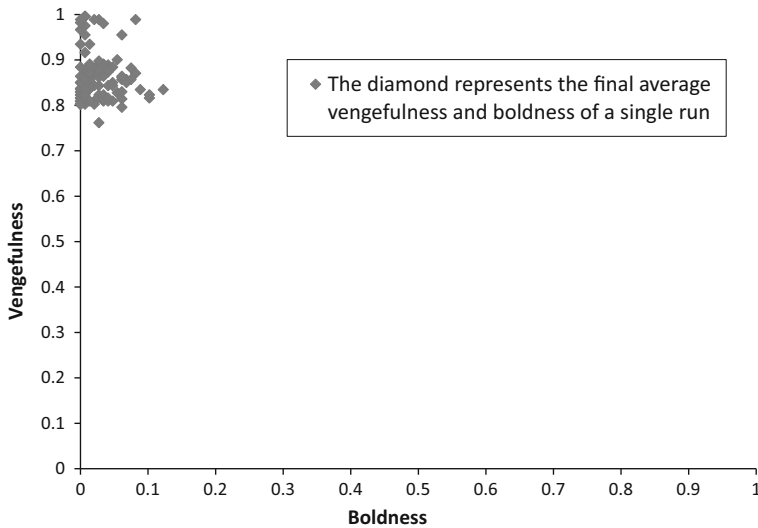
Fig. 16 Strategy improvement (with \gamma = 0.01 ), 1,000,000 timesteps
