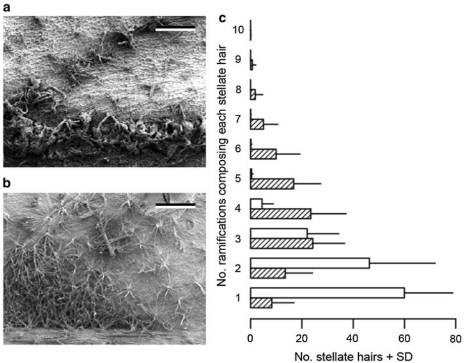
Fig. 1 a, b Stellate hairs on the surface of a VEP leaf (scanning electron microscope image), showing the a adaxial and b abaxial surfaces of the primary vein axil of the same leaf. The scale bar in each figure is 500 \mu\text{m} . c The number of ramifications of stellate hairs on the adaxial ( open bars ) and abaxial ( shaded bars ) surfaces of VEP leaves as the mean frequency with the standard deviation in 18 quadrats (5 mm \times 5 mm) from 18 leaves
