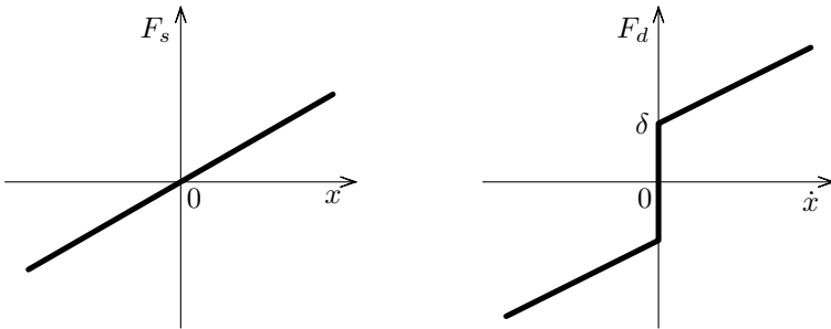
Figure 13. Relation between forces and displacement for a Bingham fluid.
