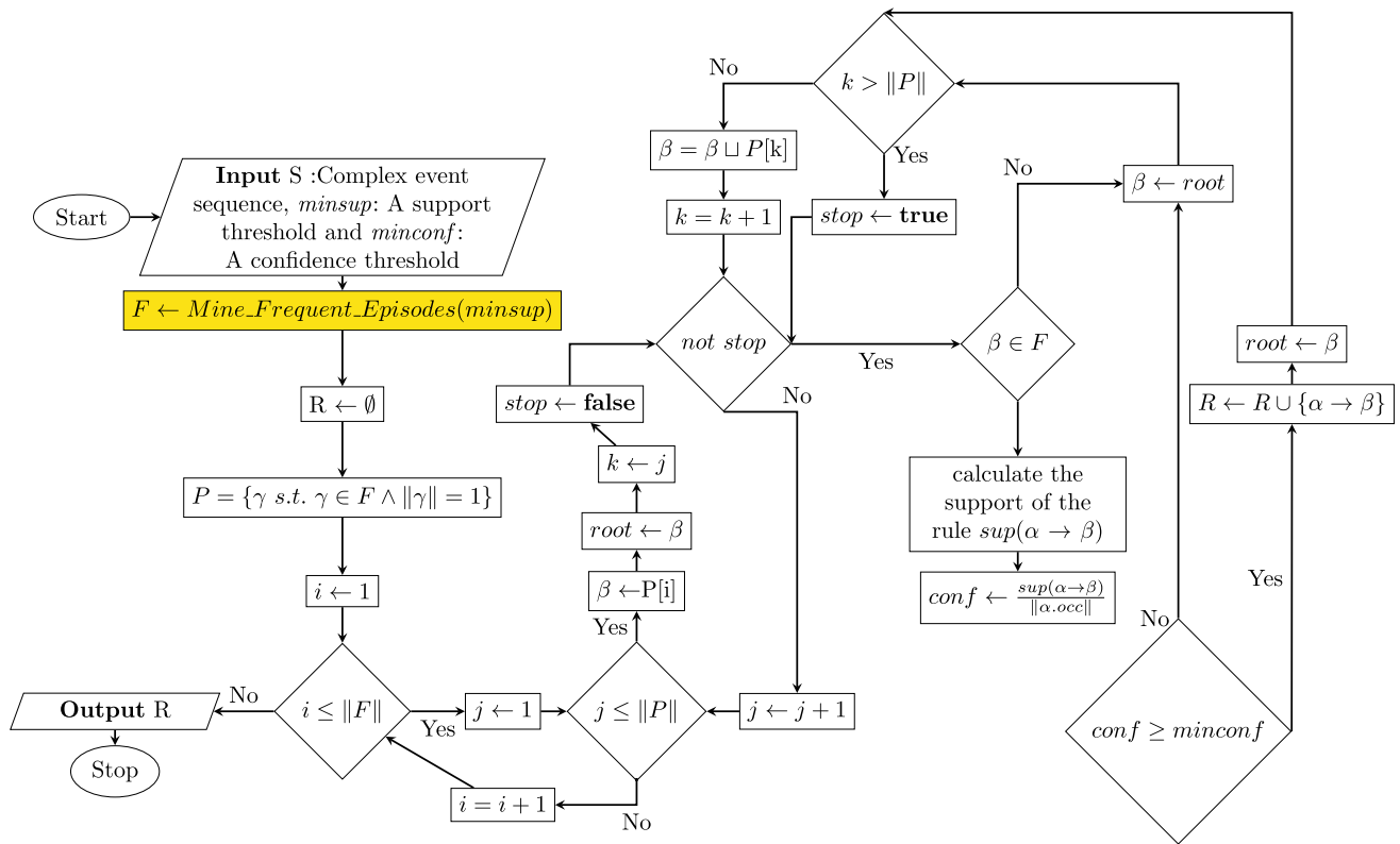
Fig. 7 Episode Rules Generation function flowchart
