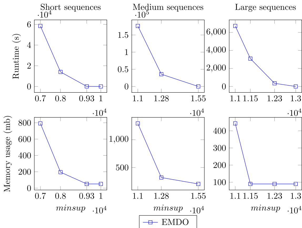
Fig. 10 Influence of minsup for frequent episode generation in terms of execution time and memory usage on synthetic data sets
