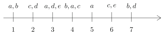
Fig. 3 A complex event sequence with 7 timestamps
