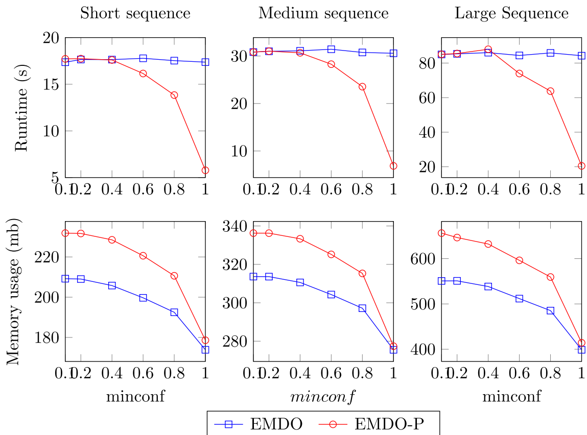
Fig. 12 Influence of minconf on execution time and memory usage of episode rules generation on synthetic datasets
