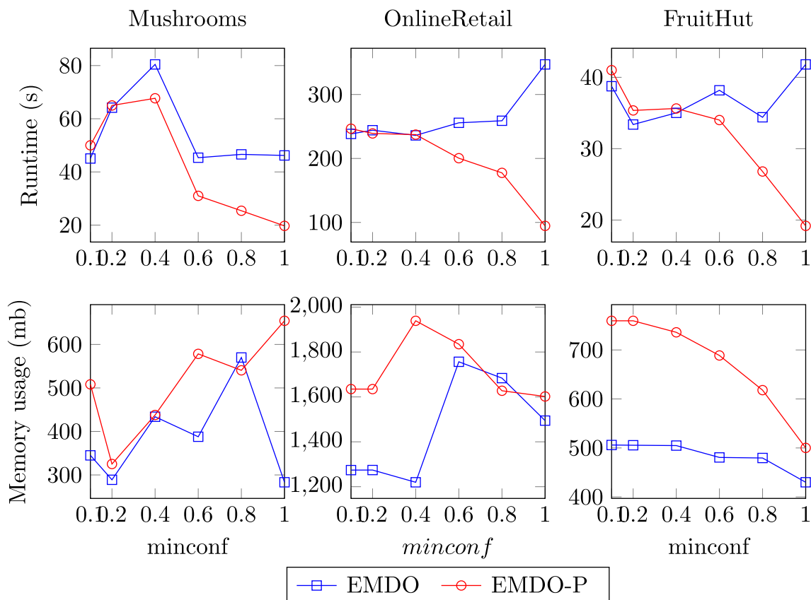
Fig. 13 Influence of minconf on execution time and memory usage of episode rules generation on real datasets
