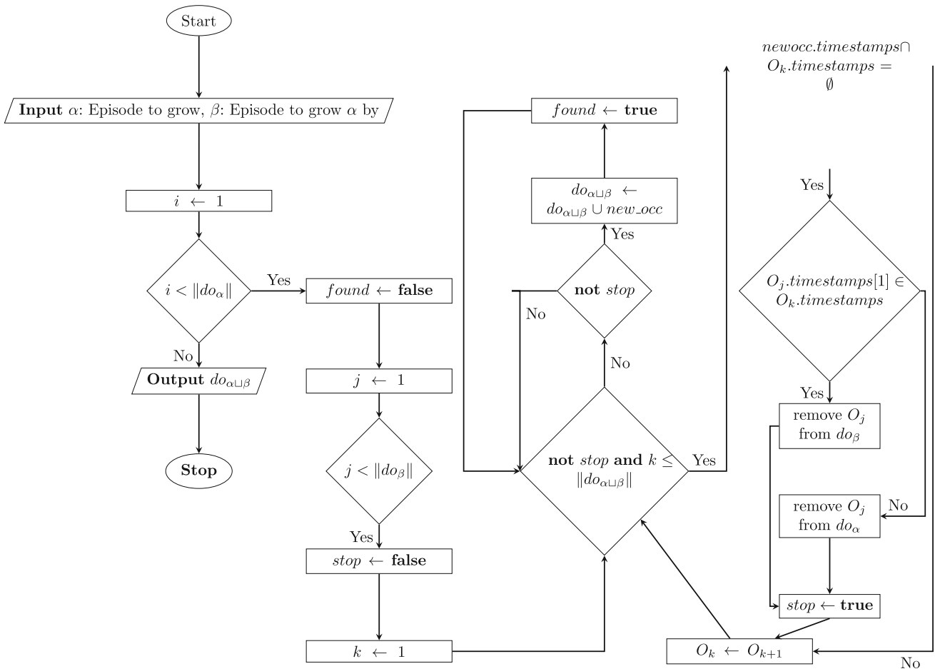
Fig. 6 Maximal set of Distinct Occurrences Recognition function flowchart
