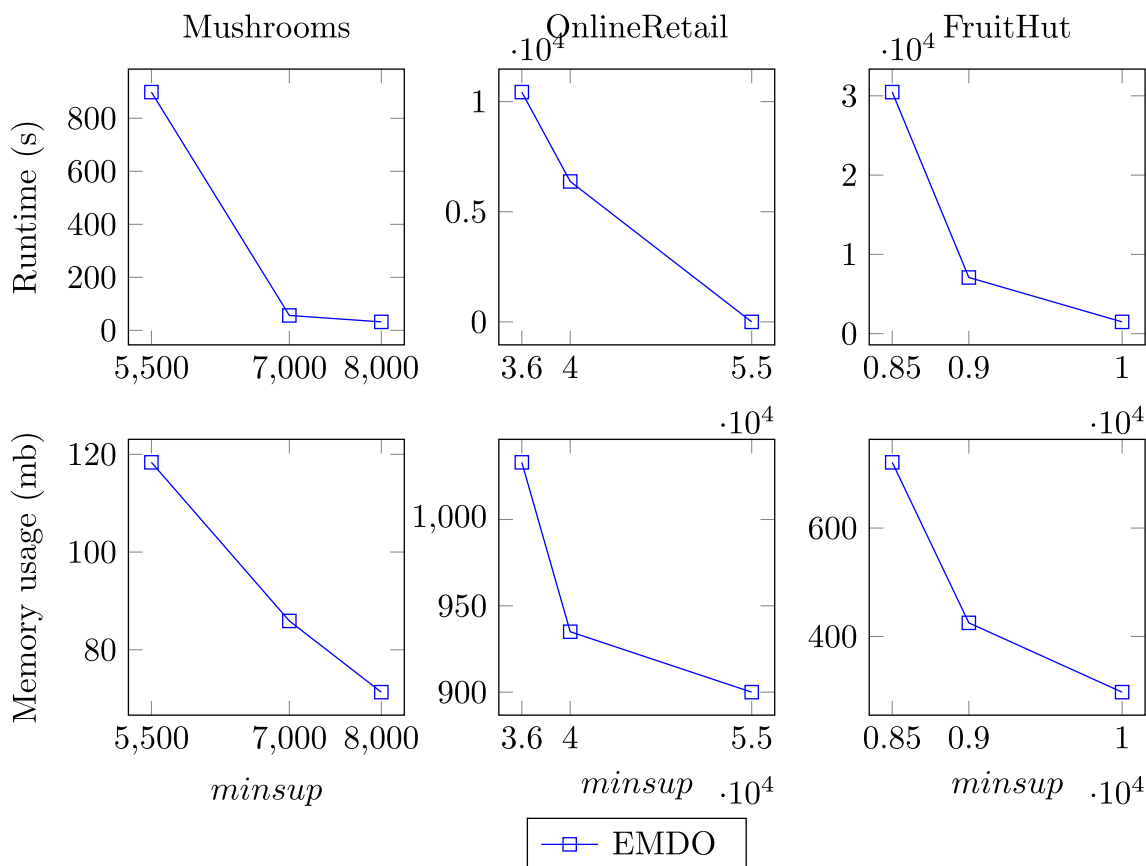
Fig. 11 Influence of minsup on execution time and memory usage on real data sets
