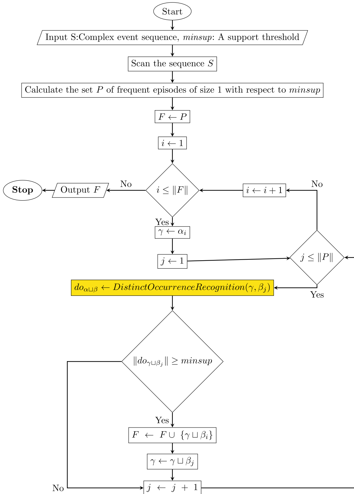
Fig. 5 Frequent Episode Generation function flowchart
