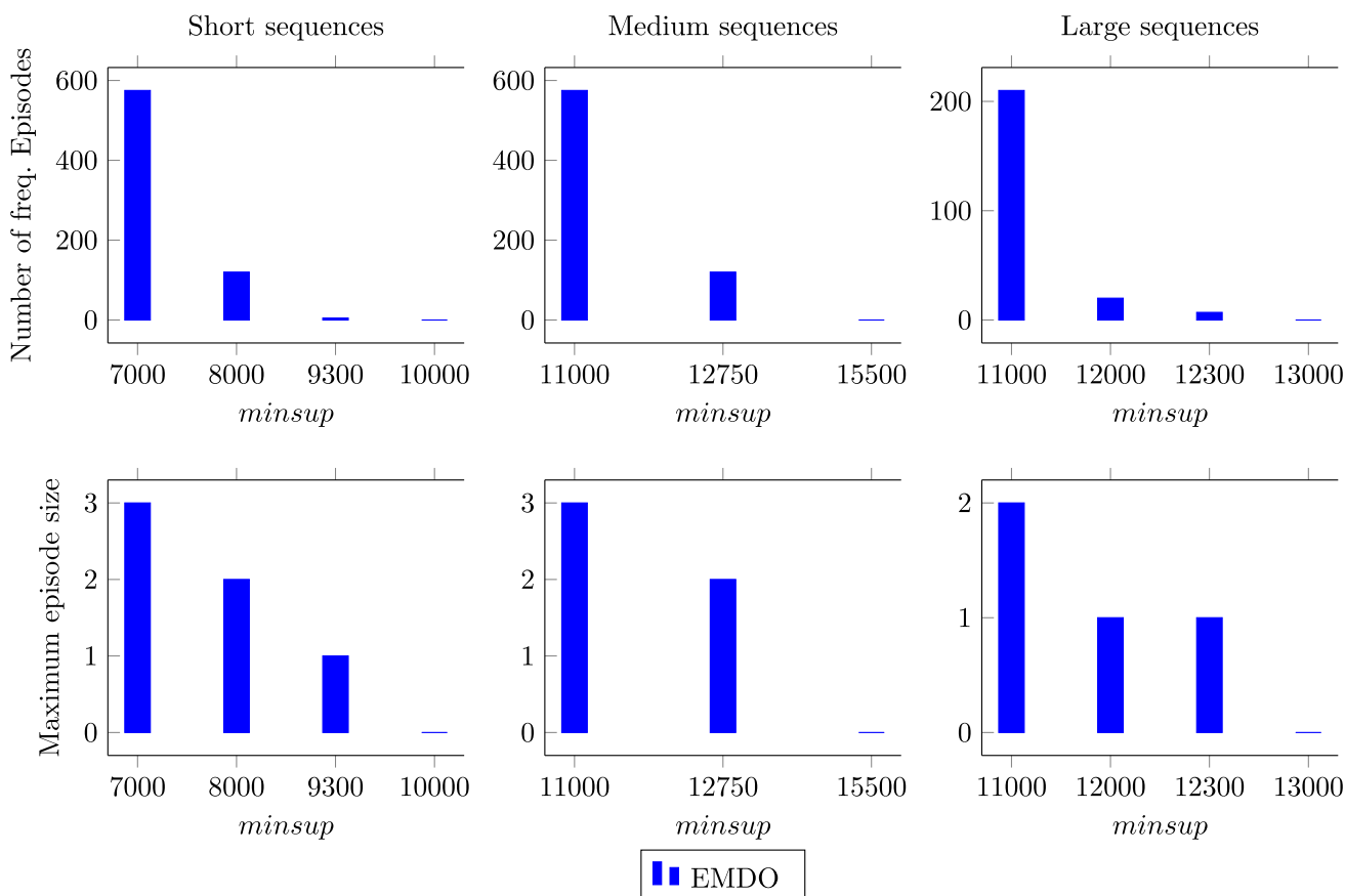
Fig. 8 Influence of minsup on the number of frequent episodes and the size of the largest episode on synthetic datasets
