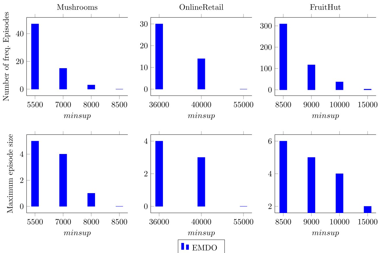
Fig. 9 Influence of minsup on the number of frequent episodes and the size of the largest episode on real datasets
