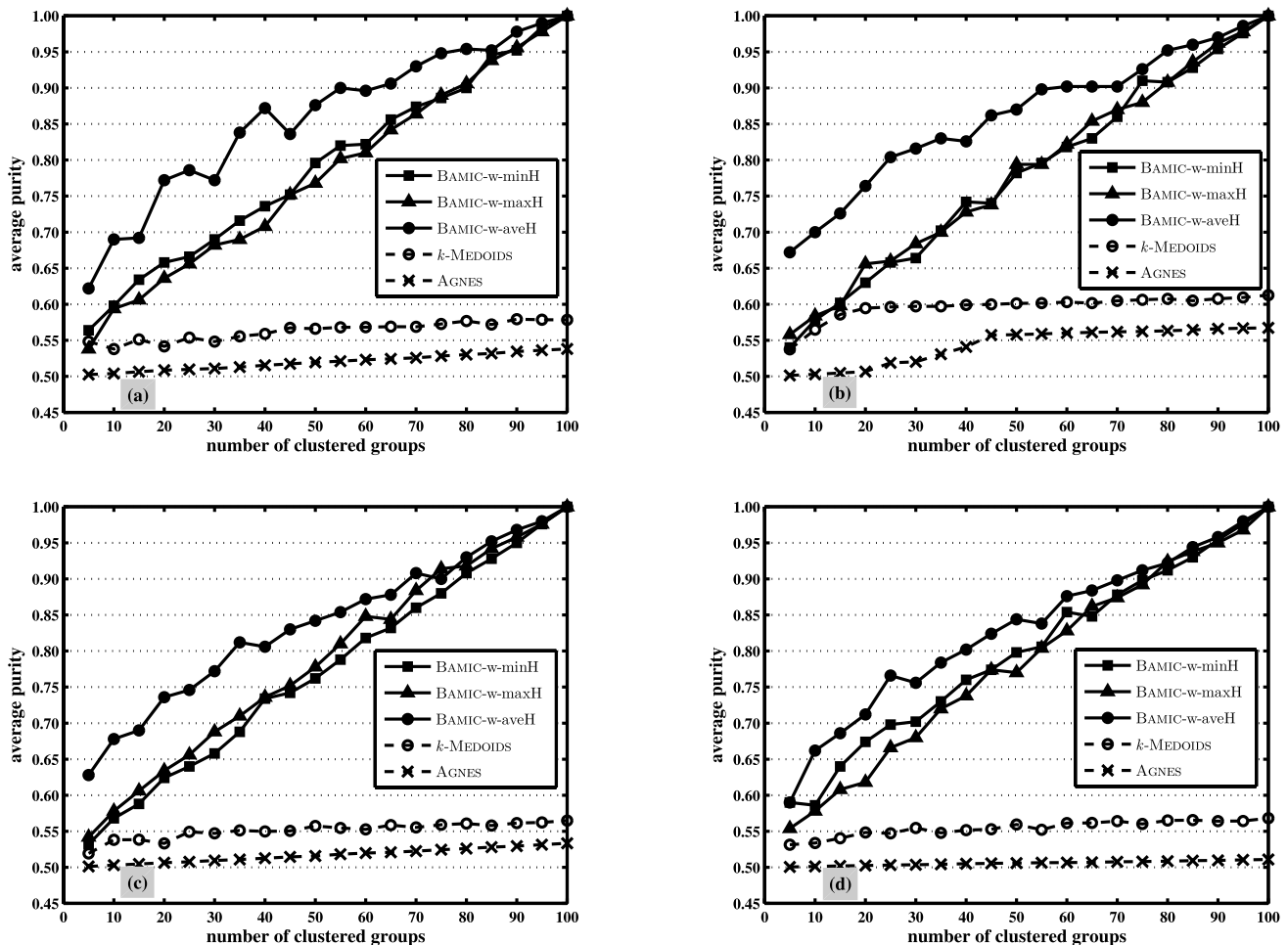
Fig. 4 The average purity of the clustering algorithm changes as the number of clustered groups increasing. a 2-5-5; b 2-10-0; c 3-5-5; d 3-5-10
