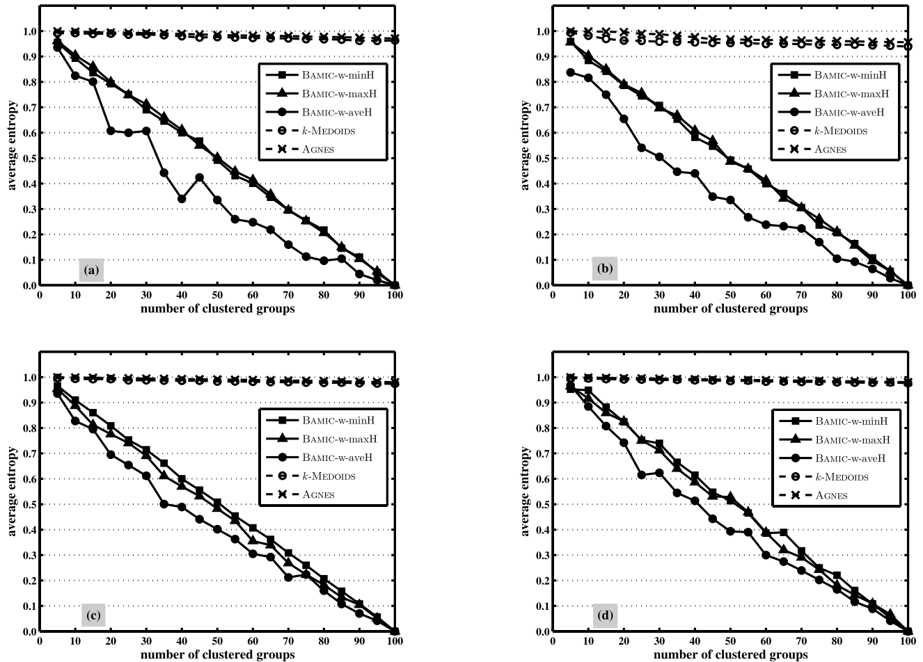
Fig. 5 The average entropy of the clustering algorithm changes as the number of clustered groups increasing. a 2-5-5; b 2-10-0; c 3-5-5; d 3-5-10
