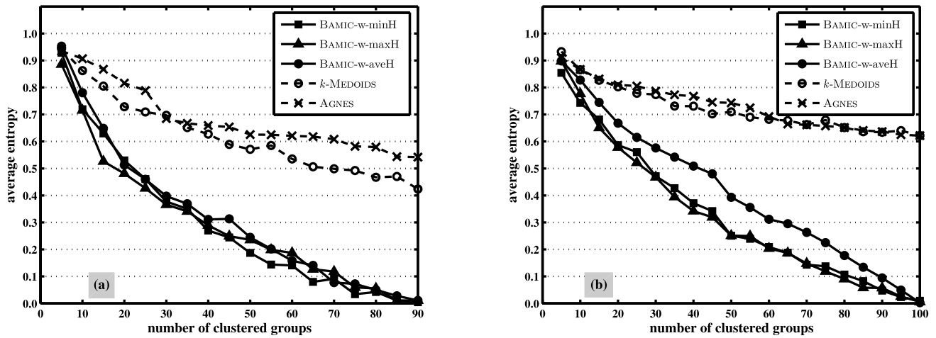
Fig. 3 The average entropy of the clustering algorithm changes as the number of clustered groups increasing. a MUSK1; b MUSK2
