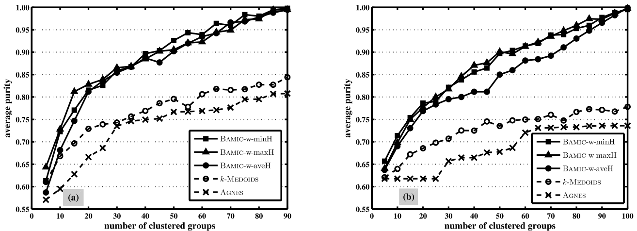
Fig. 2 The average purity of the clustering algorithm changes as the number of clustered groups increasing. a MUSK1; b MUSK2
