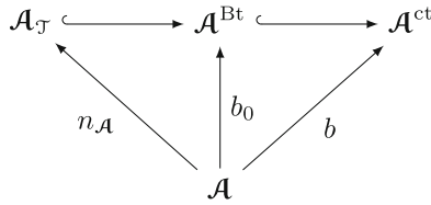
Fig. 1 The functors n_{\mathcal{A}} , b_0 and b (in the case that \mathcal{A}_{\mathcal{T}} \subseteq \mathcal{A}^{\text{Bt}} )
