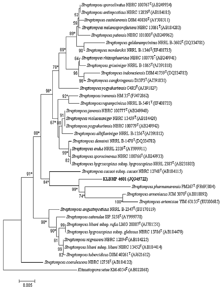
Fig. 2 Neighbour-joining tree based on almost complete 16S rRNA gene sequences (1,422 nt), showing the relationship between strain KLBMP 4601 T and its phylogenetic neighbours. Only bootstrap values above 50 %, expressed as percentages of 1,000 replications, are shown at the branch points. Kitasatospora setae KM-6054 T was used as the outgroup. Asterisks indicate that the corresponding nodes were also recovered in the maximum-parsimony and maximum-likelihood trees. Bar 0.005 substitutions per nucleotide position
