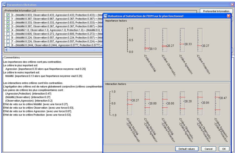
Fig. 2 Sensitivity analysis on the parameters of the capacity
