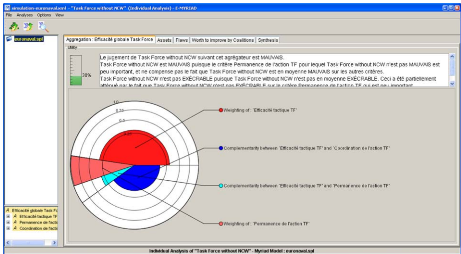
Fig. 3 Pie chart representing a 2-additive Choquet integral
