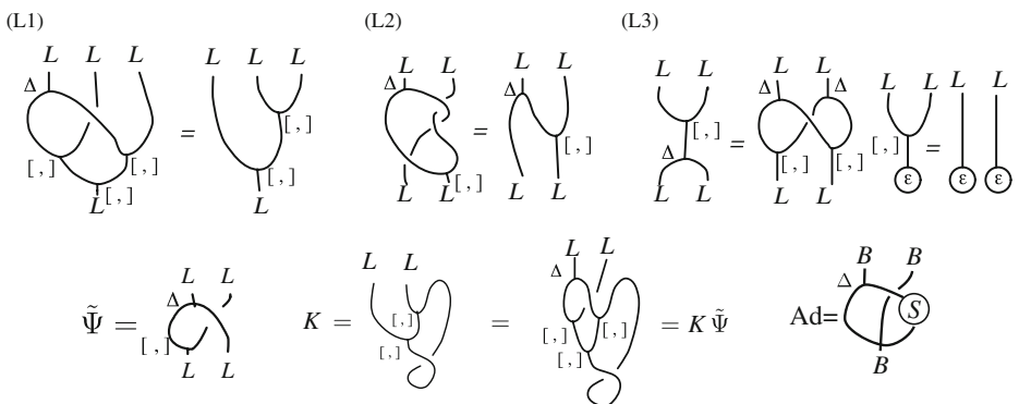
Fig. 4 Axioms of a braided-Lie algebra. Read down the page. We also recall the associated braiding \tilde{\Psi} and braided-Killing form, and the adjoint action of a braided-Hopf algebra on itself
