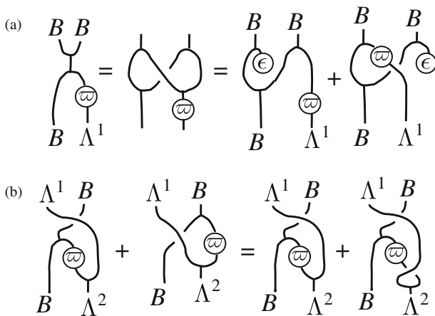
Fig. 1 Diagrams in the proof of Proposition 2.9 for quantum differentials on braided planes
