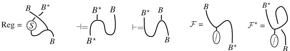
Fig. 2 Diagrammatic definitions of relevant actions, Fourier transform \mathcal{F} and adjoint Fourier transform \mathcal{F}^* on a braided-Hopf algebra B with right dual B^*
