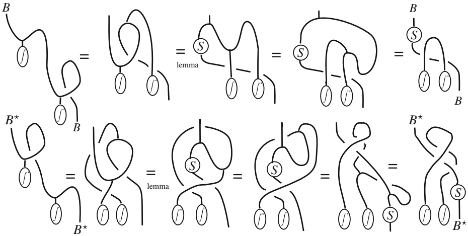
Fig. 3 Diagrammatic computations of \mathcal{F}^*\mathcal{F} and \mathcal{F}\mathcal{F}^* in Proposition 3.2
