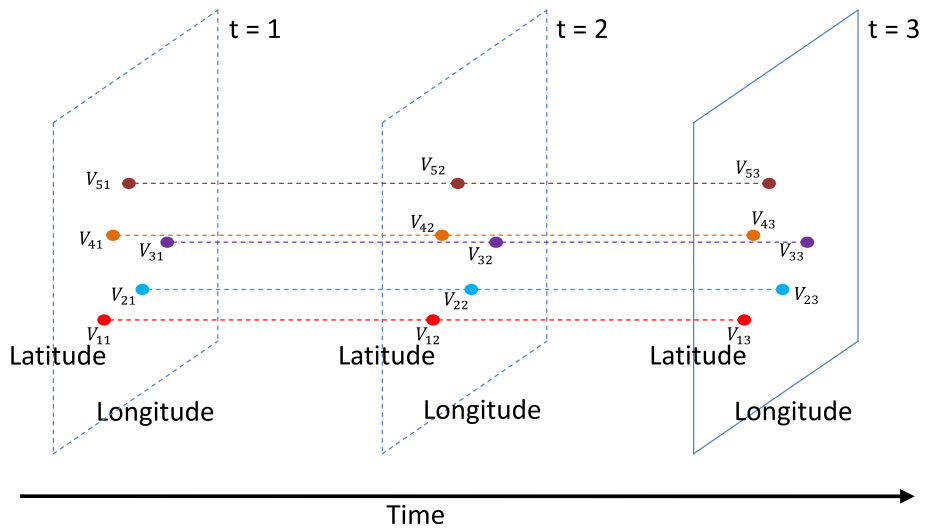
Fig. 2 Geo-referenced data items
