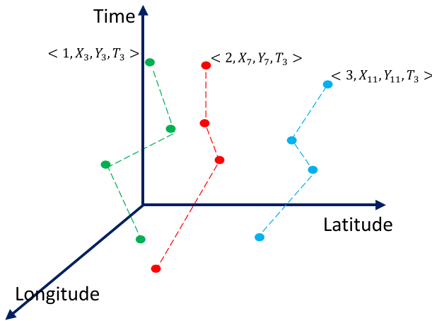
Fig. 3 Geo-referenced time series
