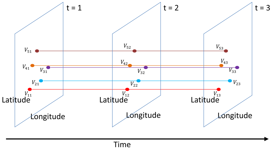
Fig. 3 Geo-referenced time series
