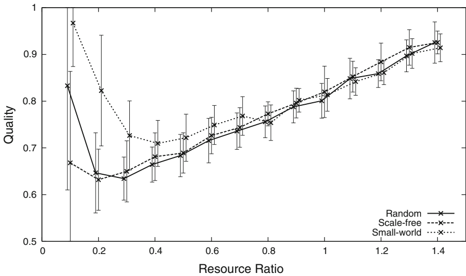
Fig. 7 The relative solution quality of GDAP is influenced by the resource ratio
