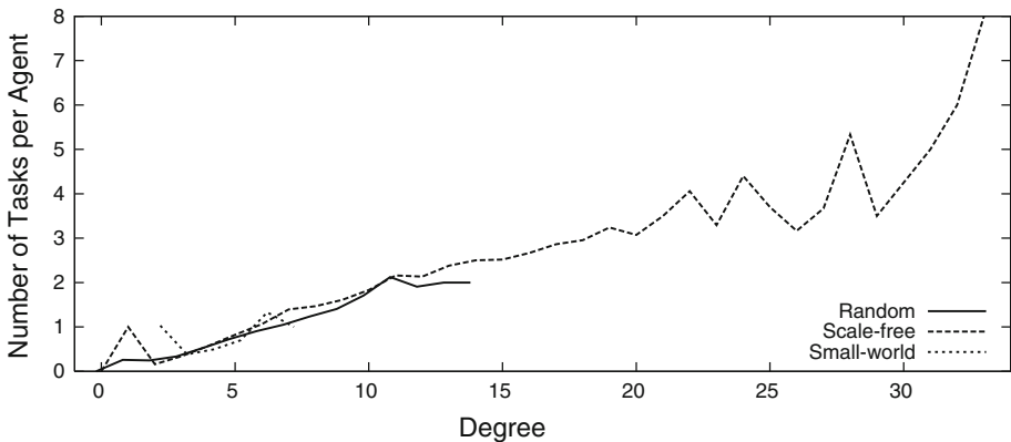
Fig. 14 The average number of tasks successfully allocated by a single agent of a given degree in networks with 10–120 agents and an average degree of 4
