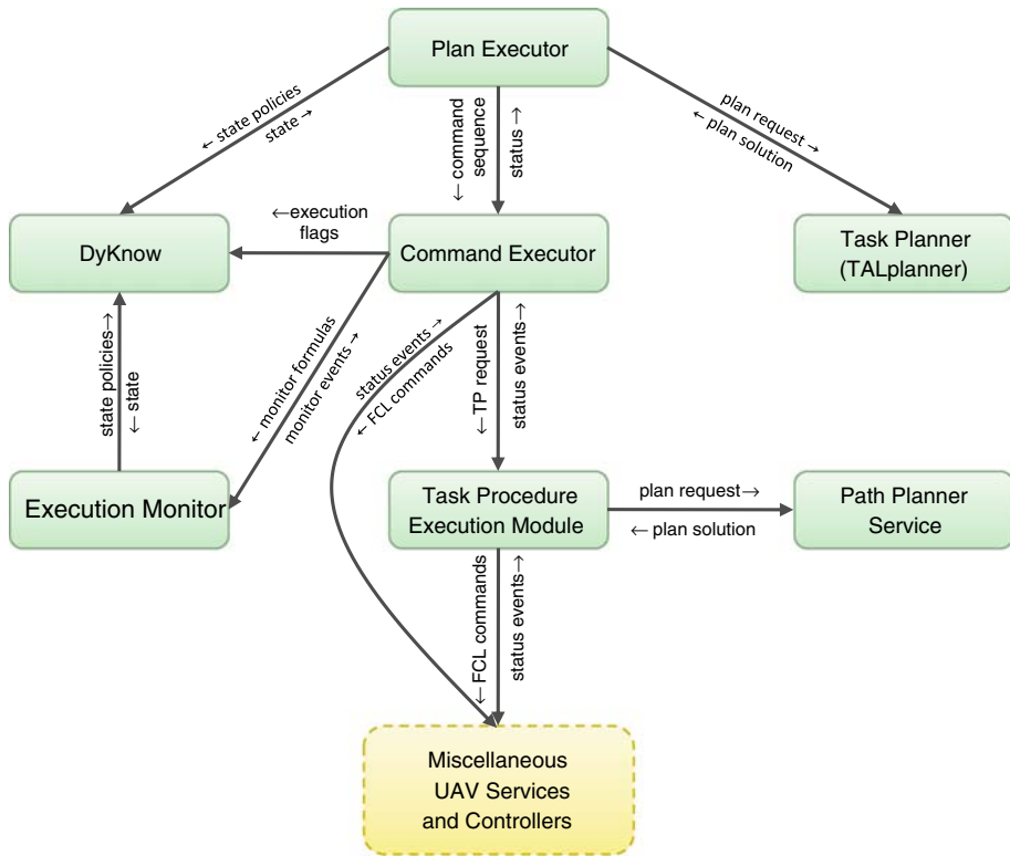
Fig. 7 Task planning and execution monitoring overview
