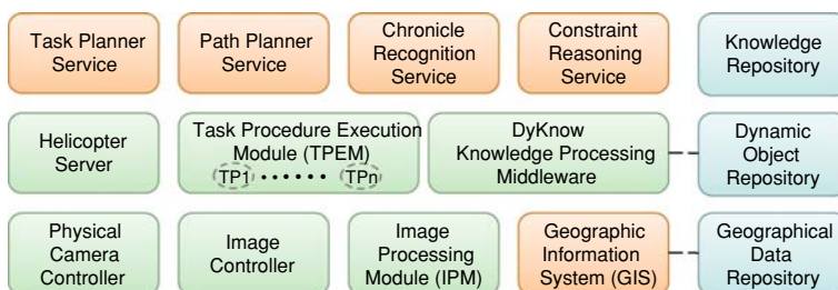
Fig. 5 Some deliberative, reactive and control services
