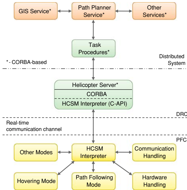
Fig. 6 Navigation subsystem and main software components
