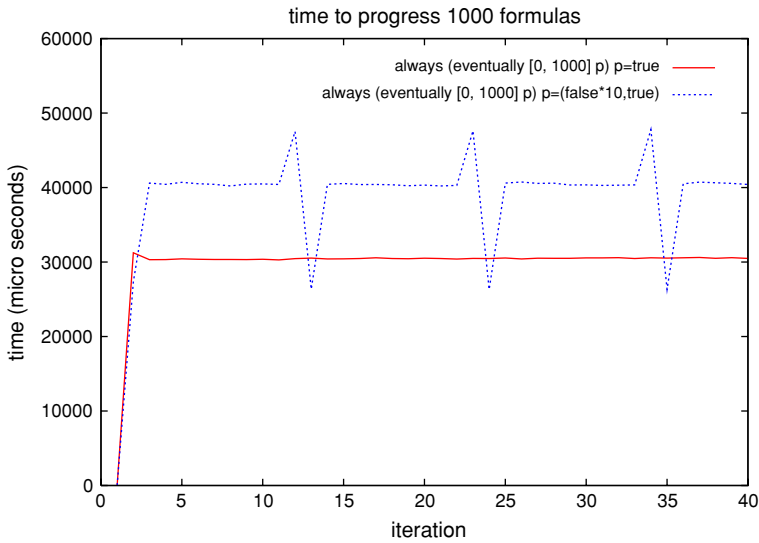
Fig. 15 Testing: always eventually (development over time)
