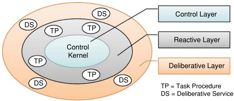
Fig. 4 The functional structure of the architecture
