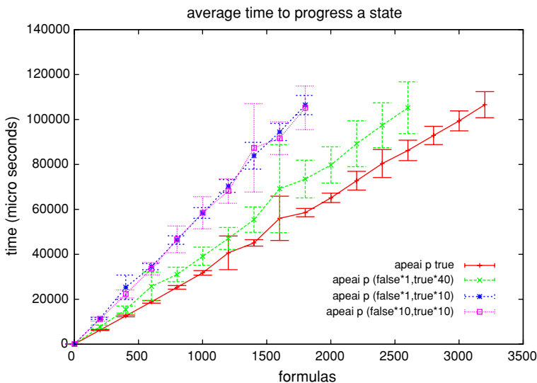
Fig. 16 Testing: always not p implies eventually always (average progression time)
