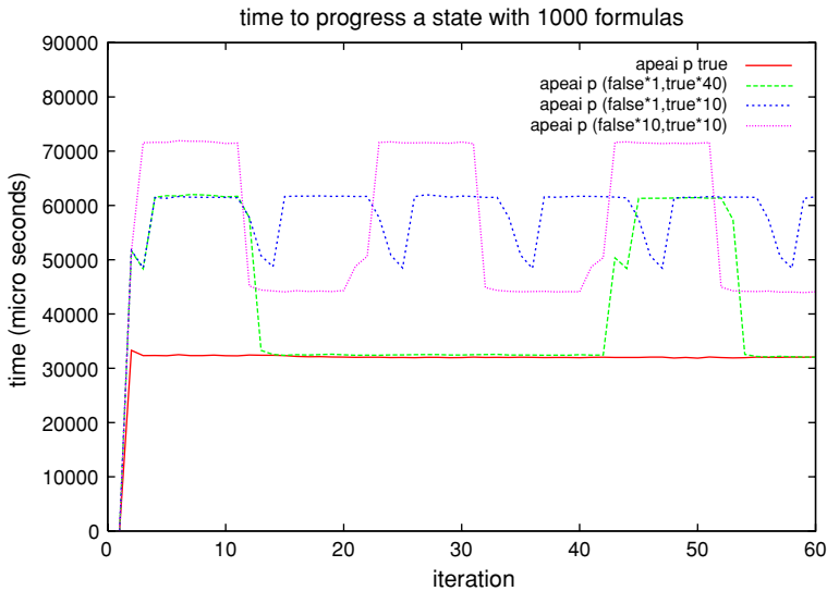
Fig. 17 Testing: always not p implies eventually always (development over time)
