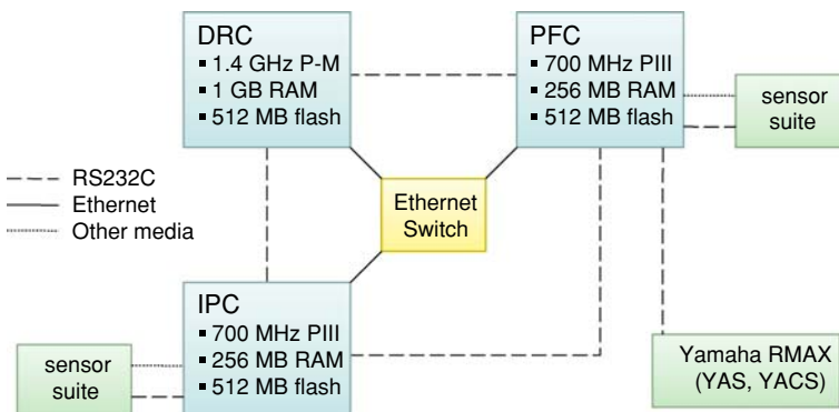
Fig. 2 On-board hardware schematic
