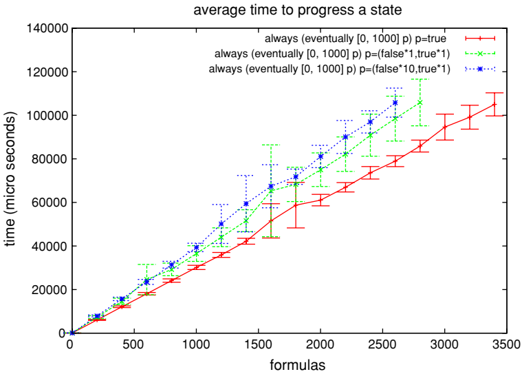
Fig. 14 Testing: always eventually (average progression time)
