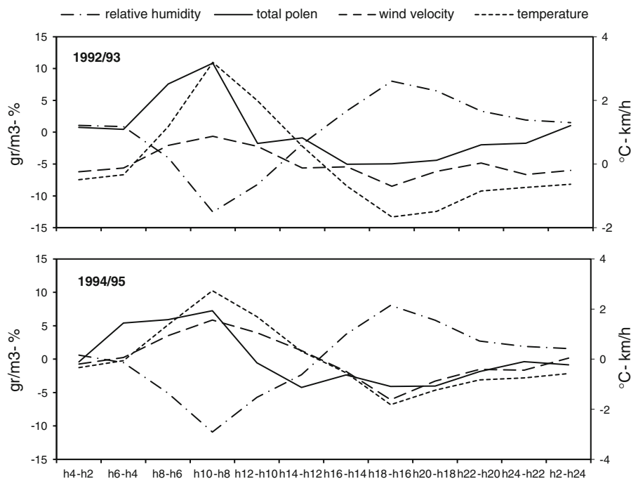
Fig. 7 Differences between consecutive hours of total pollen and meteorological variables for every period
