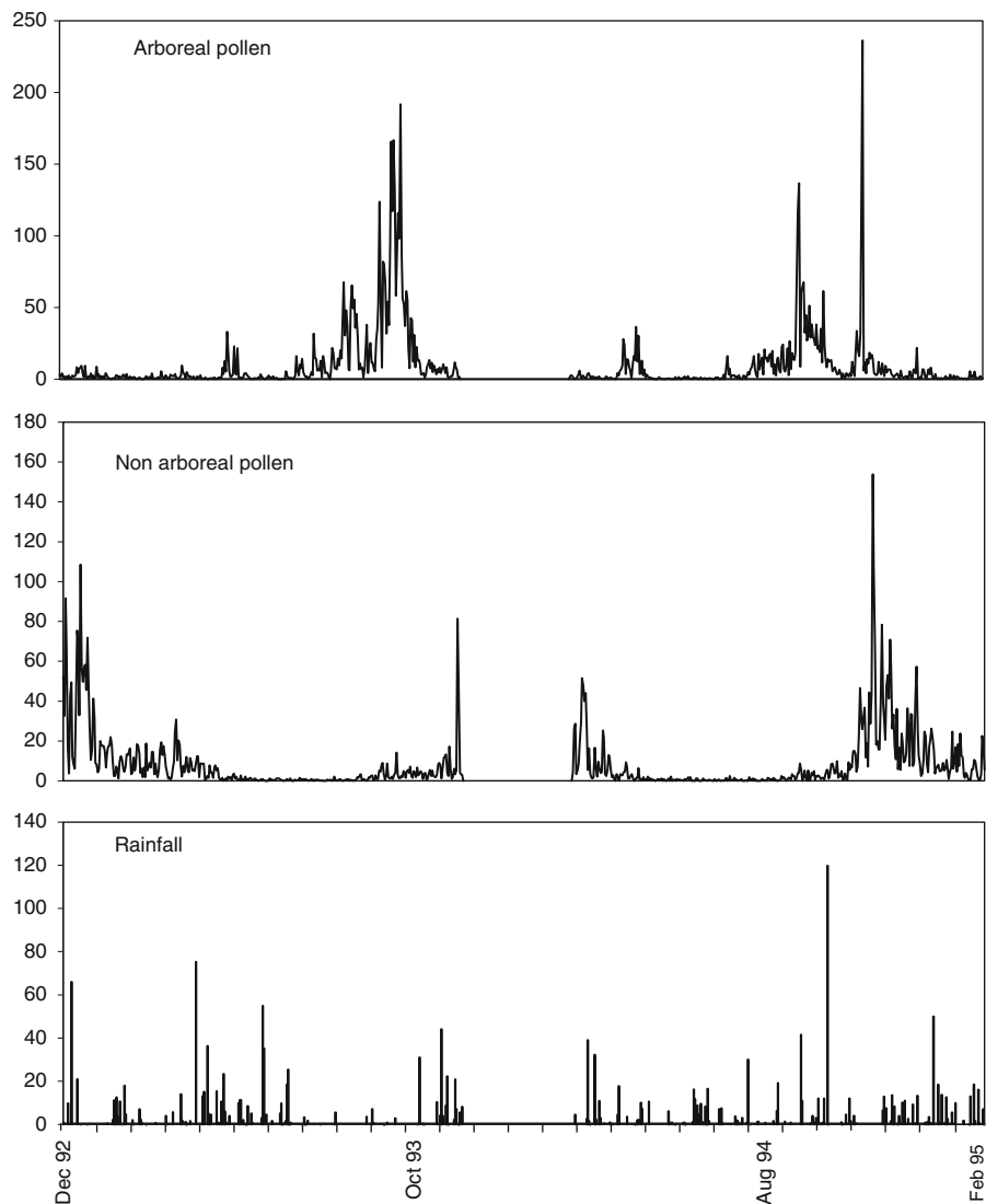
Fig. 6 Daily concentration of arboreal pollen (excluding Cupressaceae) and herbaceous pollen and daily rainfall during the periods analyzed
