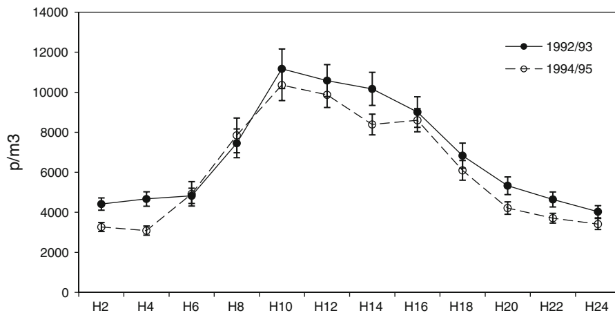
Fig. 3 Hourly concentration of total pollen for every period analyzed
