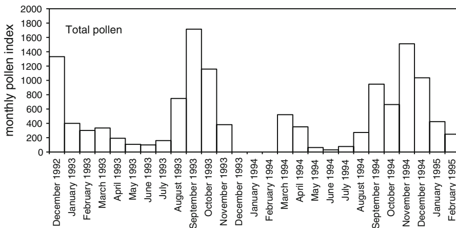
Fig. 1 Monthly sums of total pollen (excluding Cupressaceae) for every period analyzed (December 1992 to November 1993 and March 1994 to February 1995)
