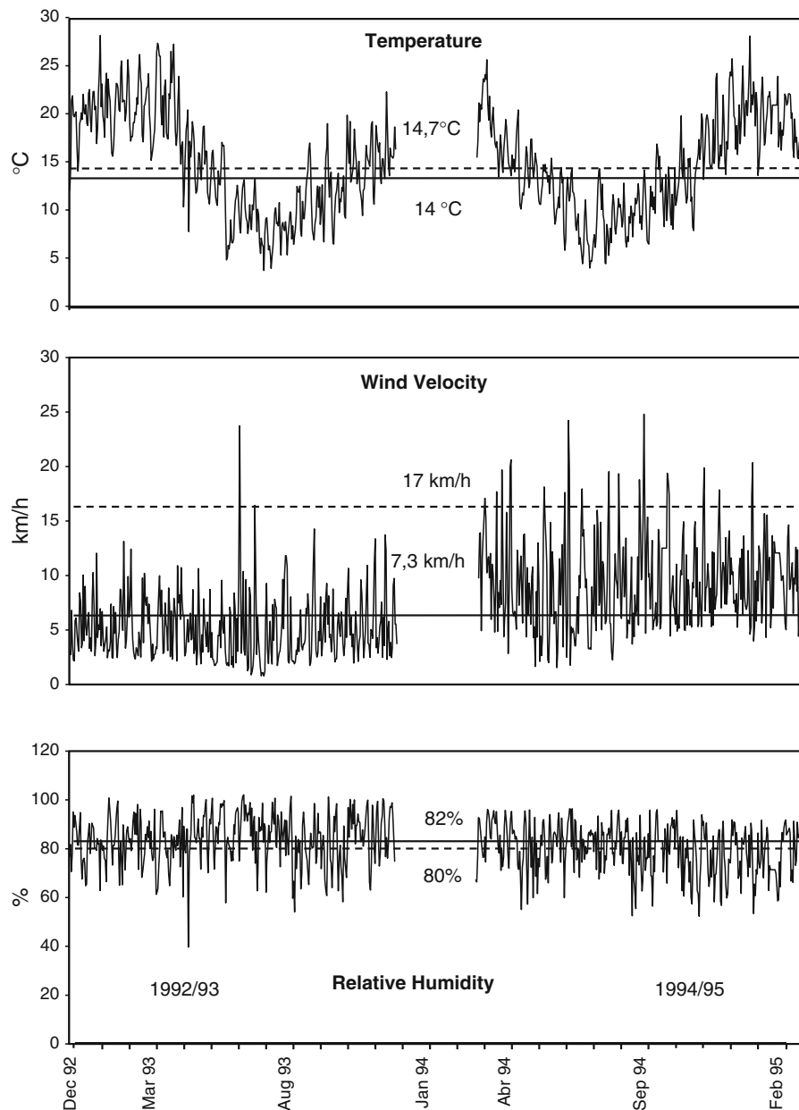
Fig. 4 Daily data of meteorological variables: temperature, wind speed and relative humidity, taken at the same site of pollen sampling. The horizontal lines indicate the mean values
