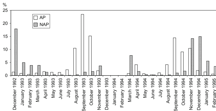
Fig. 2 Monthly percentage of arboreal pollen (AP; excluding Cupressaceae) and non-arboreal pollen (NAP) with respect to the annual total of the periods analyzed (1992/1993 and 1994/1995)
