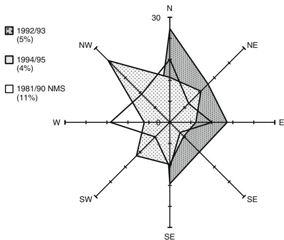
Fig. 5 Frequency (in percentage) of winds in each direction. Between parentheses, the relative proportion of hours without wind corresponding to each interval
