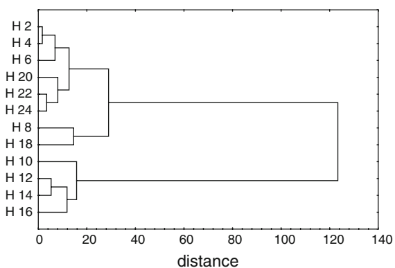
Fig. 8 Cluster analysis of hours according to pollen (total pollen) and meteorological (temperature, relative humidity and wind speed) variables of the two periods
