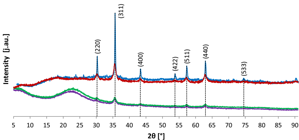
Fig. 3 XRD patterns of the synthesized nanoparticles and nanocomposites: (red line) \gamma - \text{Fe}_2\text{O}_3 -synthesized, (blue line) \gamma - \text{Fe}_2\text{O}_3 -commercial, (violet line) \gamma - \text{Fe}_2\text{O}_3/\text{SiO}_2 , (green line) \gamma - \text{Fe}_2\text{O}_3/\text{SiO}_2/\text{N} (Color figure online)
