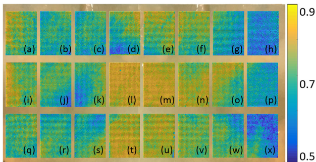
FIGURE 6. SALS analysis overlaid on full GLBP patch. Interrogation region labelling (a–x) correspond to fibre architecture detailed in Table 4.
