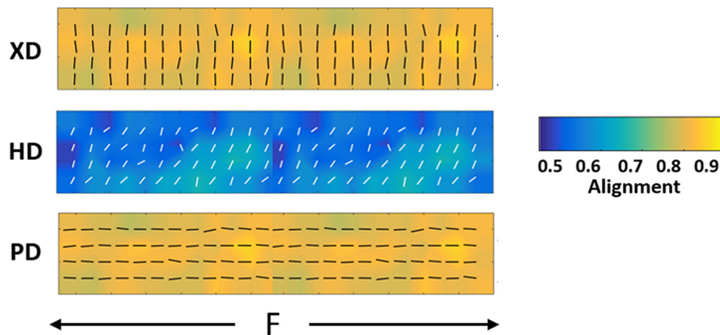
FIGURE 1. Representative SALS contour plots for one specimen from the three groups (XD, HD, PD). F direction of force applied. Colour indicates alignment (low to high; 0.5 to 0.9). White and black vectors indicate fibre angles at each location across region of analysis (6 mm \times 1 mm).
