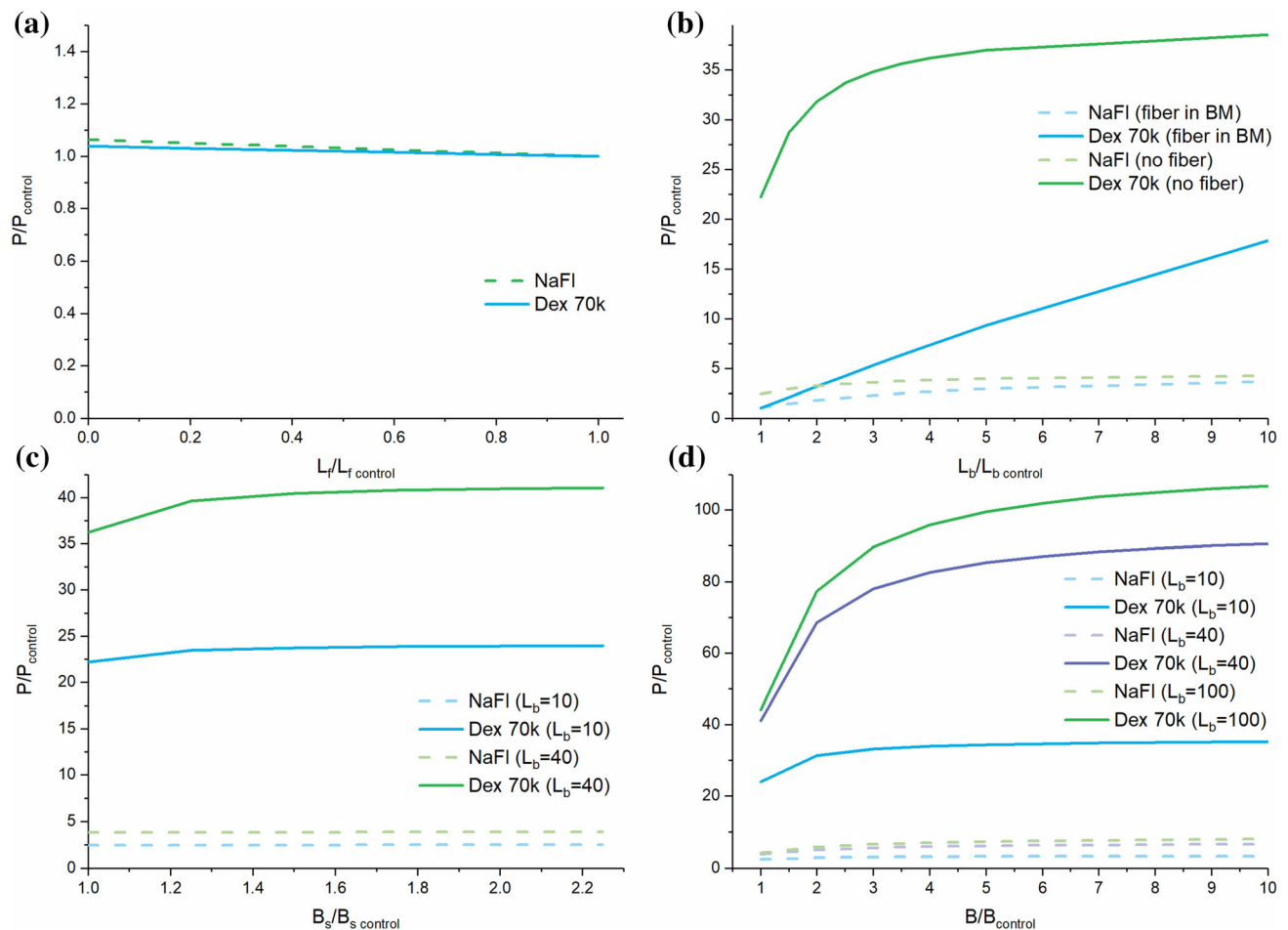
FIGURE 6. Model predictions for the BBB permeability P . For P to sodium fluorescein and FITC-dextran 70k as a function of the endothelial surface glycocalyx thickness L_f (a); as a function of the basement membrane thickness 2L_b when the surface glycocalyx is degraded and when the fiber matrix in the basement membrane is or is not degraded (b); as a function of the tight junction opening width 2B_s when the glycocalyx and the fiber matrix in the basement membrane are degraded (c); and as a function of the interendothelial cleft width 2B when the glycocalyx and the fiber matrix in the basement membrane are degraded and the junction is disrupted ( B_s = B ) (d).
