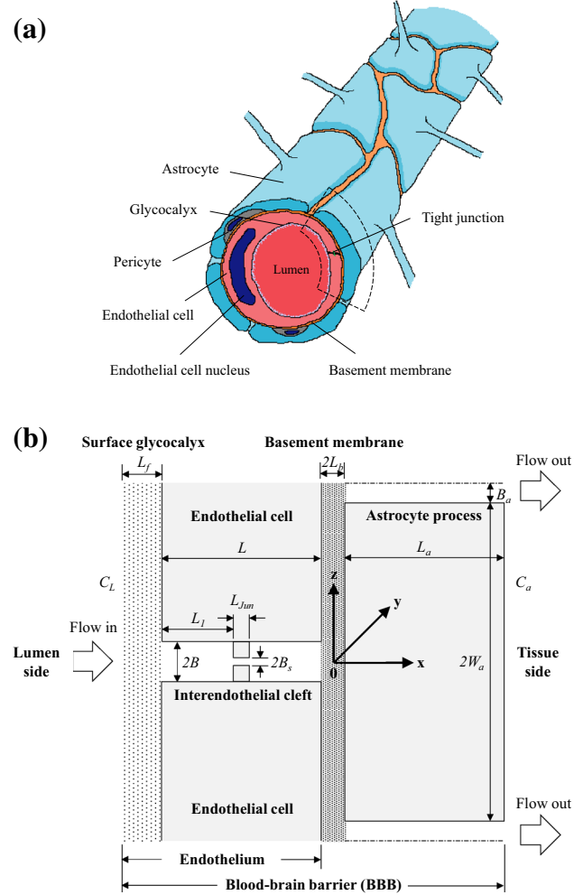
FIGURE 3. The BBB structure and the simplified model geometry for the paracellular transport. (a) Three dimensional sketch of a cerebral microvessel. Its wall (the BBB) is formed by endothelial cells, basement membrane, pericytes and astrocyte foot processes. Based on the electron microscopic observation in Farkas and Luiten. 12 (b) Simplified model geometry for the paracellular pathway of the BBB (dashed line enclosed area in a). The interendothelial cleft has a length of L and a width of 2B . The tight junction strand inside the cleft has a length of L_{\text{Jun}} and a width of 2B_s . The distance between the junction strand and luminal front of the cleft is L_1 . The thickness of the endothelial surface glycocalyx is L_f . The width of the basement membrane is 2L_b and the length of the astrocyte foot processes is 2W_a . The gap between astrocyte foot processes has a length of L_a and a width of 2B_a . Revised from Li et al. 17
