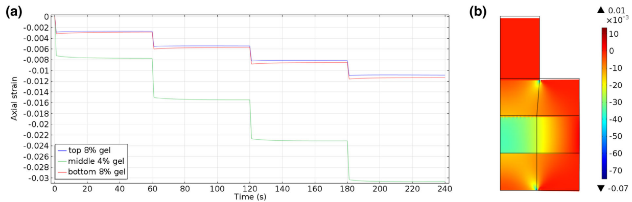
FIGURE 6. Simulated strain fields (COMSOL) in a three-layered construct as used in ultrasound elastography testing for a sequence of four 40\ \mu\text{m} ramp compressions ( 0.44\% global strain per step): (a) History of the averaged strain across each layer for the prescribed ramp compressions. (b) Strain map at the end of the fourth step ( 160\ \mu\text{m} , 1.78\% global strain, 240\ \text{s} test time).
