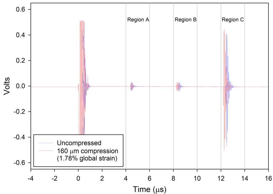
FIGURE 4. Ultrasound echoes from the internal and external boundaries of the three-layered hydrogel construct under 0 (blue) and 160 \mu\text{m} compression (red). The other three steps (40, 80, and 120 \mu\text{m} ) are not shown in this figure. The maximum value of the normalized cross-correlation function was used to calculate the time delay between pre- and post-compression signals within a ROI. Three ROI windows (a 4–6 \mu\text{s} , b 8–10 \mu\text{s} , and c 12–14 \mu\text{s} ) were selected to track the time shifts of the echoes reflected from the interfaces of the bottom to the middle gel, the middle to the top gel and the top gel to the acoustic reflector, respectively.
