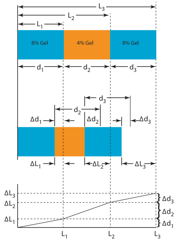
FIGURE 3. Measurement of strain in three springs connected in series. Top and middle: configurations of 3-layer hydrogel constructs pre- and post-compression. L_i are the uncompressed free length to the interfaces in a global coordinate system; d_i are the local thickness of each gel. \Delta L_i are the changes in L_i , \Delta d_i are the changes in d_i , both after compression. Bottom: local strains are the slopes of each segment the trace in the graph of deflection ( \Delta L ) vs. free length ( L ).
