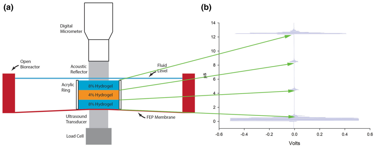
FIGURE 2. (a) Schematic illustration of the custom designed elastography test rig: a three-layered construct was formed from three agarose hydrogels which were cast individually, stacked up, and then held by an acrylic ring (16 mm outer diameter, 12.7 mm inner diameter, 10 mm height) to prevent sliding. The top and bottom layers were 8% gels and the middle was a 4% gel. The gel stack was placed in a bioreactor chamber (without the top membrane, for convenience) and sandwiched between a micrometer-positioned acoustic reflector and the ultrasound transducer. A load cell was in-line with the transducer. (b) The ultrasound A-mode echogram of the three-layered construct before compression. The first, (lowermost) waveform is the reflection from the interface between the bioreactor membrane and the bottom 8% gel. The second waveform is the reflection from the lower interface between the bottom 8% gel and the middle 4% gel. The third waveform is the reflection from the upper interface between the middle 4% gel and the top 8% gel. The upper-most waveform is the reflection from the interface between the top 8% gel and the acoustic reflector.
