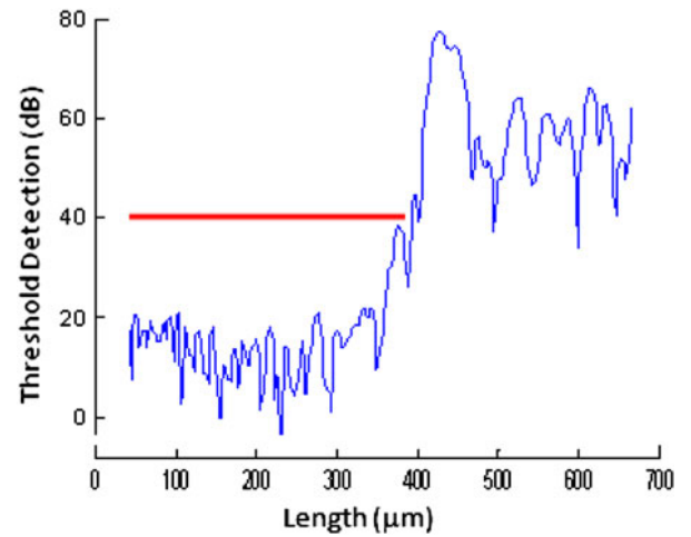
FIGURE 1. Plot diagram of the SAM, showing the detection of the device surface (red line) after setting the threshold detection safely above the signal of the water.
