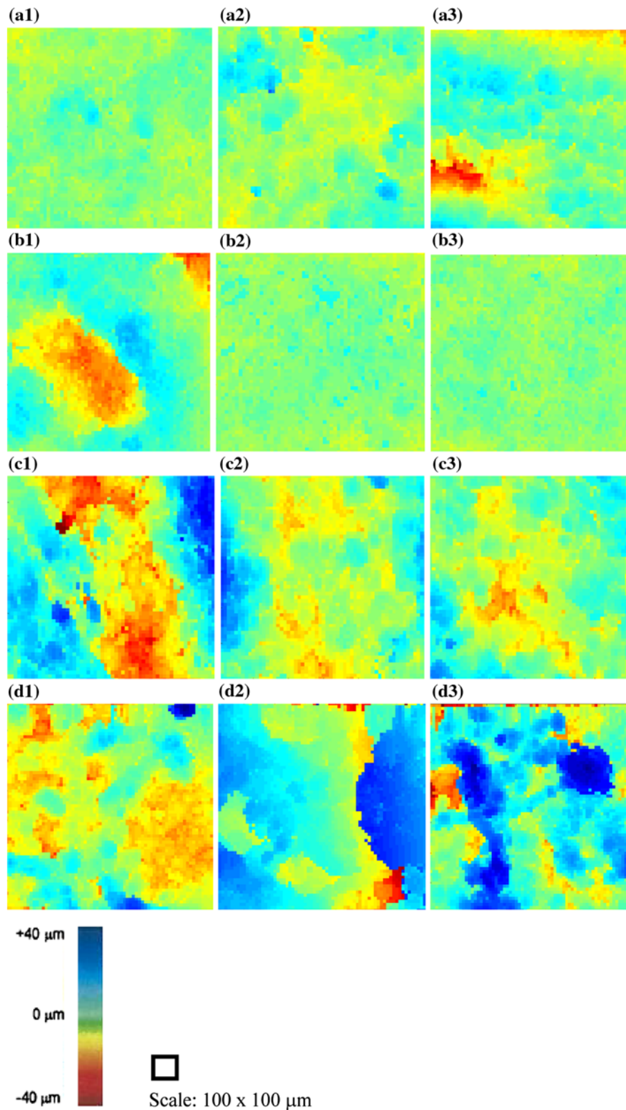
FIGURE 4. RMS profilometry images for each scan performed on the thermally non-stressed (a–b) and stressed (c–d) devices. For the latter, there is higher variation in the surface features—presumably from the thermal stress fractionating the keratinized layer. With the non-stressed devices, there is little variation in the surface profiles, characteristic of the uniformity of the keratin layer on their surfaces.
