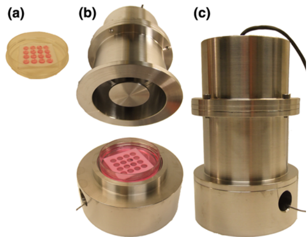
FIGURE 2. Bioreactor setup: (a) Petri dish with 1.5 mm thick PTFE spacer holding up to 16 constructs in position for loading. (b) Constructs surrounded by medium in bioreactor for loading. (c) Bioreactor during dynamic compression.
