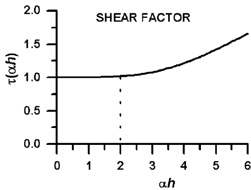
FIGURE 1. The shear factor predicts homogenous wall shear stress in the PPFC. The shear factor T(\alpha h) is equal to 1.0 when \alpha h < 2 . Under this condition, the fluid flow regime is quasi-steady, which induces a homogenous wall shear stress.
