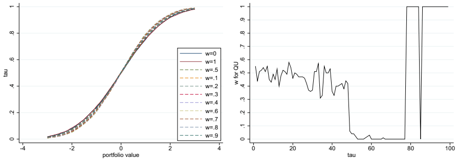
Fig. 18 (X, Y) \sim N(0, \Sigma) with \Sigma = [1 \ 0.5; 0.5 \ 1] . Left box plots CDF of S_w . Right box plots QP portfolio selection
