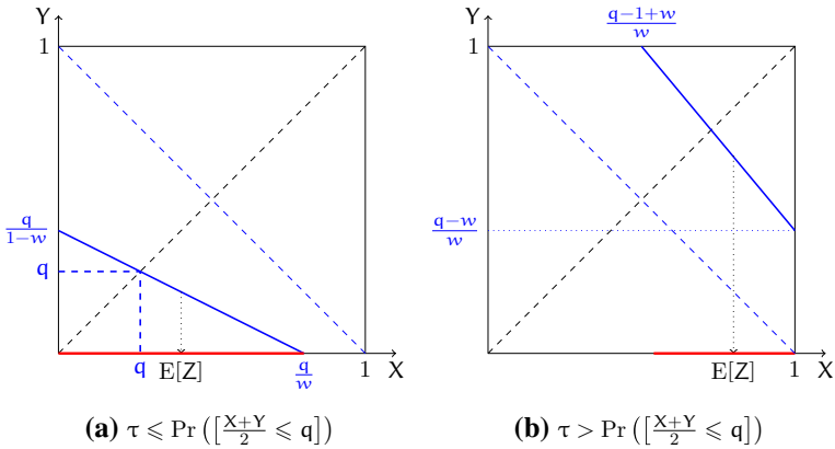
Fig. 5 An illustration of Z for the case \mathcal{J}_X = \mathcal{J}_Y = [0, 1]
