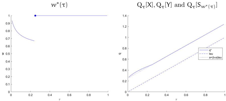
Fig. 4 Illustration of Example 3.9—Optimal w^* for X \sim \mathcal{U}(0.25, 1.25) and Y \sim \mathcal{U}(0, 1)
