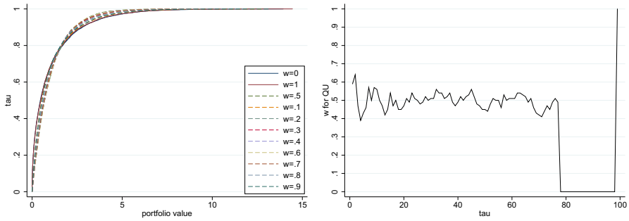
Fig. 15 X, Y \sim \chi^2_1 . Left box plots the CDF of S_w . Right box plots QP portfolio selection
