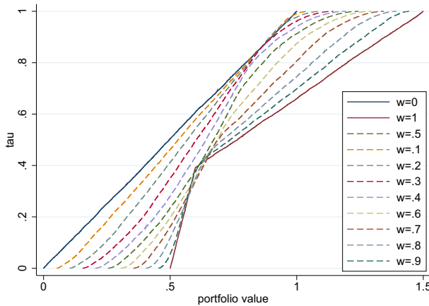
Fig. 2 CDF of S_w = wX + (1 - w)Y indexed by w \in [0, 1] when (X, Y) are defined in the Example 3.7
