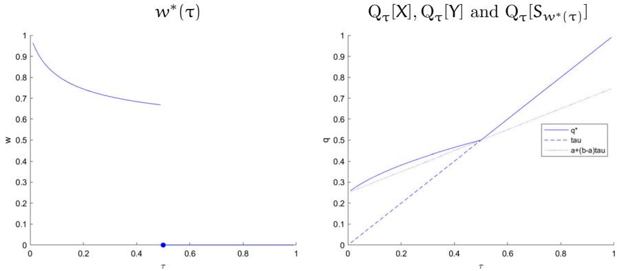
Fig. 3 Illustration of Example 3.8—Optimal w^* for X \sim \mathcal{U}(0.25, 0.75) and Y \sim \mathcal{U}(0, 1)
