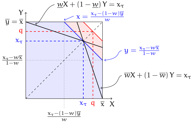
Fig. 13 Illustration for the proof of Theorem 3: the case of \tau close to 1
