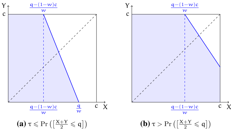
Fig. 14 An illustration of Z for the case \mathcal{J}_X = \mathcal{J}_Y = [0, c] . The blue area has probability \tau
