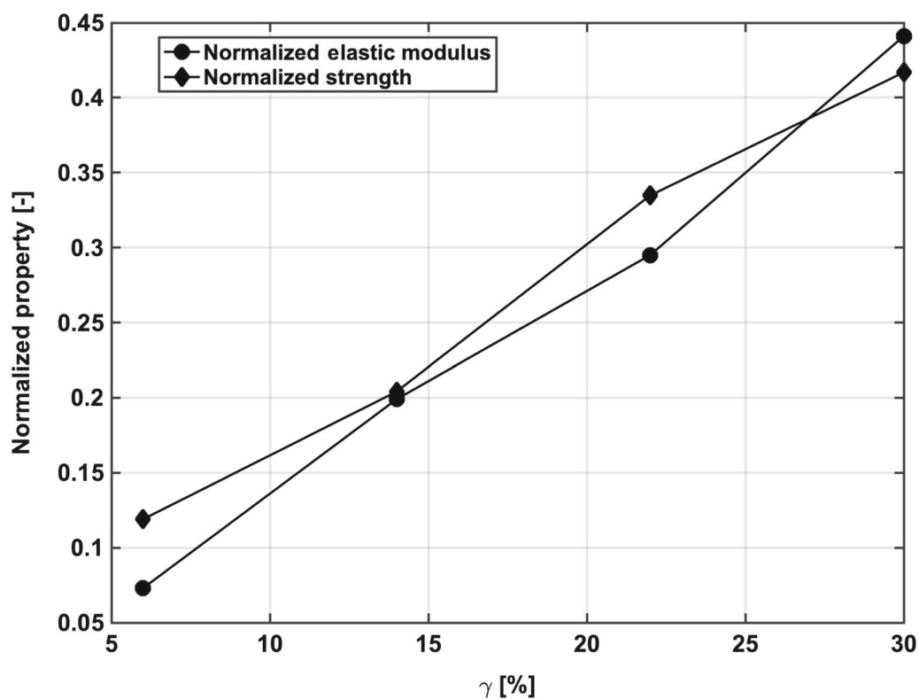
Fig. 7 Normalized elastic modulus and normalized strength as a function of the fiber compenetration \gamma
