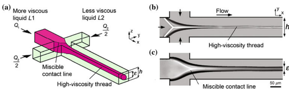
Fig. 14 Formation of threads of a core fluid lubricated with a miscible fluid. a Schematic three-dimensional view, b , c experimental micrographs of miscible contact lines for different flow rate ratios
