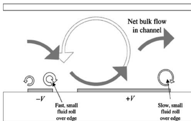
Fig. 3 Schematic diagram of AC electroosmotic flow in an asymmetric electrode array. The asymmetry leads to fluid rolls of different sizes over each electrode resulting in a net fluid flow. Reprinted with permission from Ramos et al. 2003
