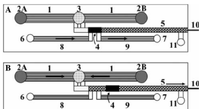
Fig. 12 Schematic representation of a microfluidic LC system. 1 Pumping channels; 2A, 2B eluent inlet reservoirs; 3 eluent outlet reservoir; 4 double-T injector that contains the sample plug; 5 separation channel; 6 sample reservoir; 7 sample waste reservoir; 8 sample inlet channels; 9 sample outlet channels; 10 ESI capillary emitter; 11 LC waste reservoir. a Sample loading; b sample analysis. Arrows indicate the main flow pattern through the system. Reprinted with permission from Lazar et al. 2006
