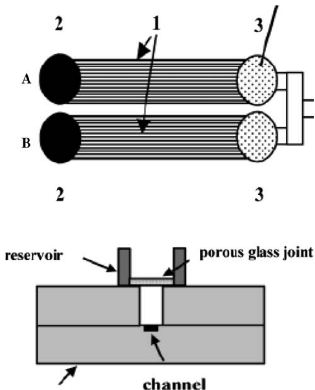
Fig. 6 Open-channel EOP. 1 Open-channel EOP, 2 micropump inlet reservoir, and 3 micropump outlet reservoir. The bottom figure shows an expanded view of reservoir 3 containing the porous glass disk. Reprinted with permission from Lazar and Karger 2002
