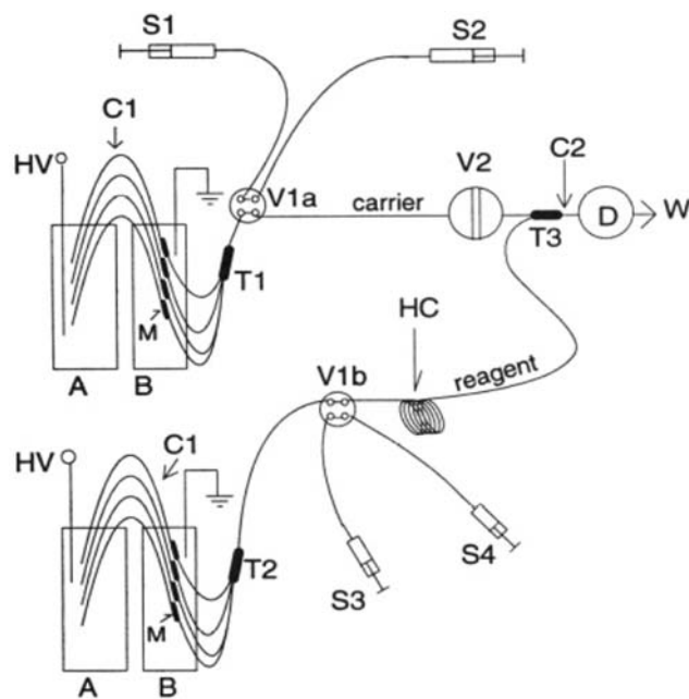
Fig. 8 Schematic diagram of two-line FIA system with EOF pumping; B, pump electrolyte solution container; T1, T2, capillary unions; V1a and V1b, four-way valve stacks a and b; S1 and S3, syringes holding pump buffer solution; S2 and S4, syringes respectively holding carrier and reagent solutions; HC, reagent holding coil; T3, low-volume tee union. Reprinted with permission from Dasgupta and Liu 1994
