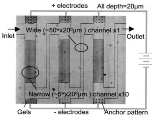
Fig. 7 Photograph of fabricated cascade-type EOP. Reprinted with permission from Takamura et al. 2003
