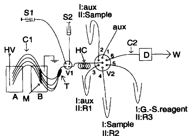
Fig. 9 Schematic diagram of capillary format SIA system. HV High-voltage power supply; A , B pumping electrolyte solution containers; M membrane joint; C1 pumping capillary; T 4 \times 1 union; HC holding coil; V1 four-way valve; S1 , S2 syringes; V2 6 \times 1 selector valve; R1 , R2 , R3 reagents; aux, unused auxiliary solution port. Reprinted with permission from Liu and Dasgupta 1994
