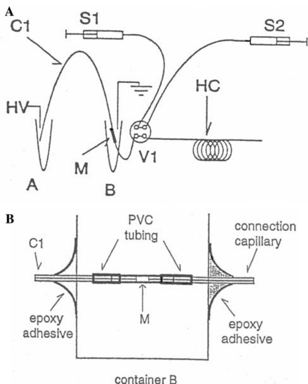
Fig. 5 Schematic diagram of an stand-alone EOP: a schematic configuration of an stand-alone EOP; b detailed structure of a membrane joint. A Pump electrolyte container; B vial housing M and containing the same solution as A ; HV high-voltage power supply; C1 pumping capillary; M membrane; V1 four-way valve; S1 and S2 syringes respectively holding pump buffer solution and reagent solutions; HC reagent holding coil. Reprinted with permission from Dasgupta and Liu 1994
