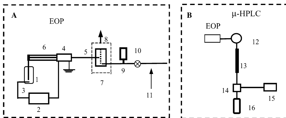
Fig. 11 Schematic diagram of the one-stage EOP and the \mu -HPLC system. a The EOP system: 1 solvent reservoir, covered with an insulating sheath; 2 high-voltage direct current source module; 3 Pt wire; 4 hollow electrode (grounded); 5 capillary conduit; 6 packed columns, three packed columns connected in parallel; 7 gas releasing device (8 representation of gas leaving direction); 9 liquid pressure
