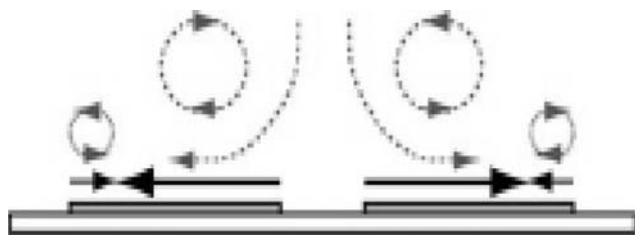
Fig. 2 Schematic diagram of AC electroosmotic flow in a symmetric electrode array. Surface slip at electrodes, and resulting fluid streamlines are represented with solid and broken lines , respectively. Reprinted with permission from Urbanski et al. 2006
