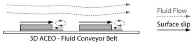
Fig. 4 Schematic diagram of AC electroosmotic flow in a 3D stepped electrode array. Surface slip at electrodes, and resulting fluid streamlines are represented with solid and broken lines , respectively. Reprinted with permission from Urbanski et al. 2006
