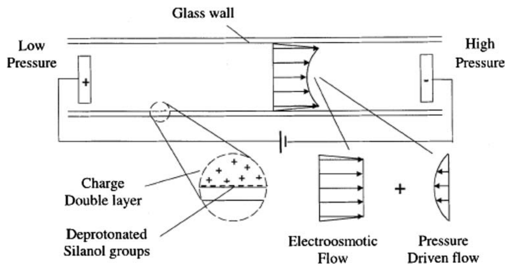
Fig. 1 Schematic illustration of electric double layer and principle of EO flow. In EOF, mobile ions in the diffuse counter-ion layer of the electric double layer are driven by an externally applied electrical field. These moving ions drag along bulk liquid through viscous force interaction. The net flow is the superposition of EOF and pressure forces. Reprinted with permission from Chen and Santiago 2002
