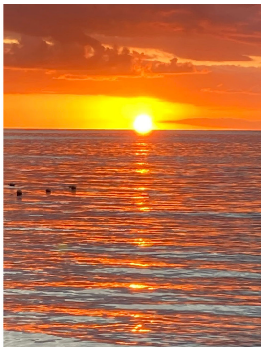
Fig. 5 This image cartoons the idea of the author that space-time and electromagnetism are the manifestations of cosmic energy. As such the photons follow the distinct geometrical field orientation of space time curving and electromagnetism to collect, transform and propagate quantum based entangled impulses of energy to interact with the retina of the observer (man, pathologist, physicist, reader, writer, etc.). As such appear world, life, nature and joy. May your surgery be a strong and positive part of it. Image obtained at sea level. Immune staining has not been applied
