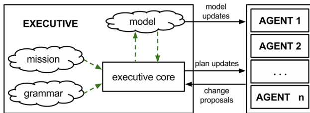
Fig. 3 The executive holds the mission of the robot, the grammar and the current model. With each world model modification proposed by any of the agents, the executive updates the plan correspondingly
