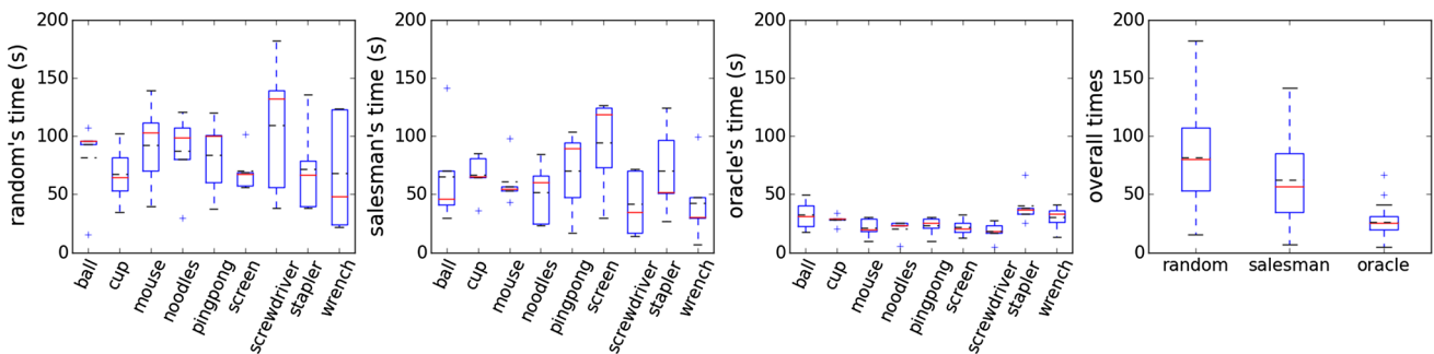
Fig. 14 Boxplots showing the time spent by the robot when approaching the tables containing the different objects, from left to right of the random, travelling salesman and oracle policies. The
