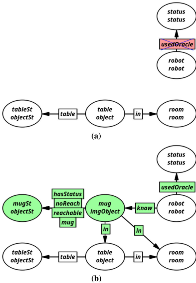
Fig. 6 The action “ imagineMugInPosition ” describes the preconditions to imagine a mug (a) and how performing such action would affect the internal world model (b). a Action “ imagineMugInPosition ”: LHS. b Action “ imagineMugInPosition ”: RHS
