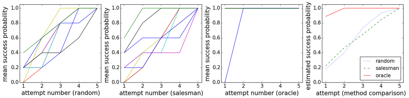
Fig. 13 Mean accumulated success for different objects, from left to right of the random, travelling salesman and oracle policies. The graphic on the rightmost position compares the general mean
