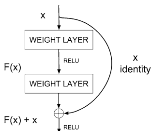
Fig. 10 A building block of the residual learning process in the DNN used in the experiments, proposed in He et al. (2015)
