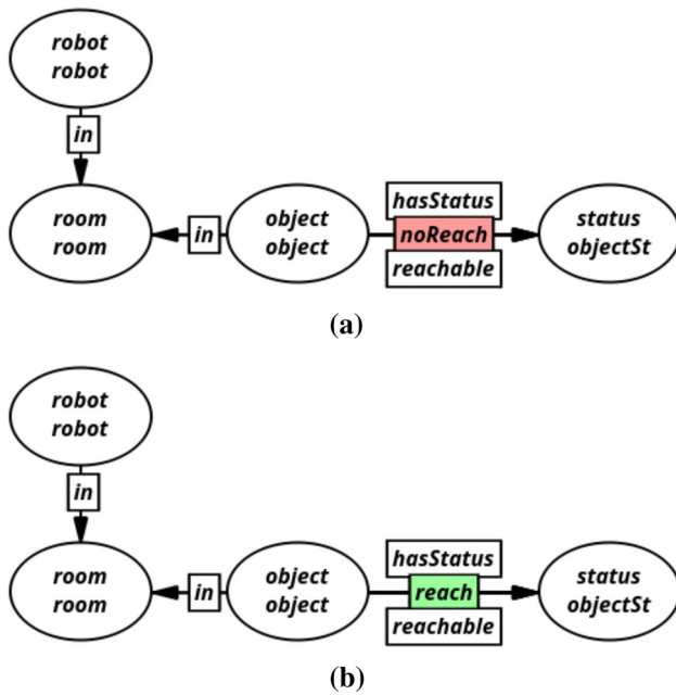
Fig. 4 The action “setObjectReach” describes the preconditions to make an object reachable (a) and how performing such action would affect the internal world model (b). a Action “setObjectReach”: LHS. b Action “setObjectReach”: RHS
