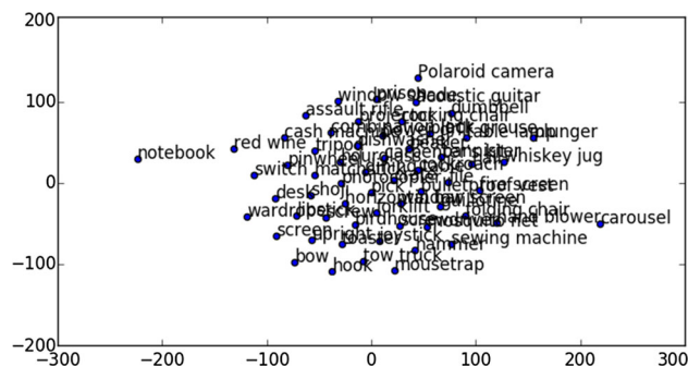
Fig. 11 A 2D plot of the vector representations of labels obtained for a table containing office objects
