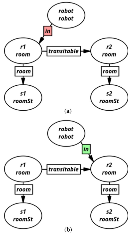
Fig. 5 The action “changeRoom” describes the preconditions to make the robot move from a room to another adjacent room (a) and how performing such action affects the internal world model (b). a Action “changeRoom”: LHS. b Action “changeRoom”: RHS
