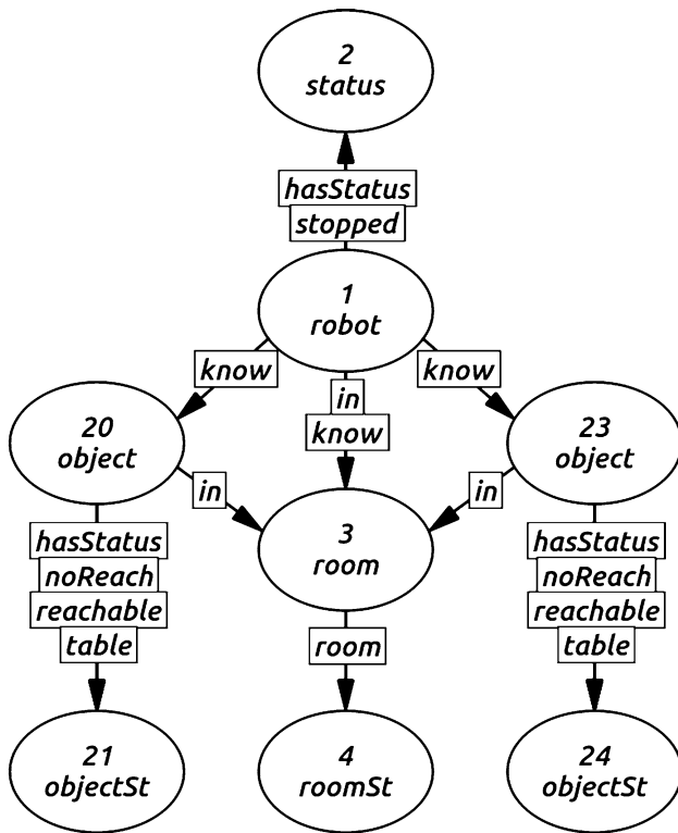
Fig. 2 AGM models represent the world as understood by the robots. The nodes of these graphs represent symbols. Each of them contains two strings: the upper one is a unique identifier and the one in the bottom represents the type of the node. Edges, which can be interpreted as binary predicates, can represent any kind of symbolic property. In this particular case, it is shown the model of a robot which is stopped and—to the knowledge of the robot—is located in a room with two more tables. Nodes and edges can hold string-to-string mappings used to store geometric information
