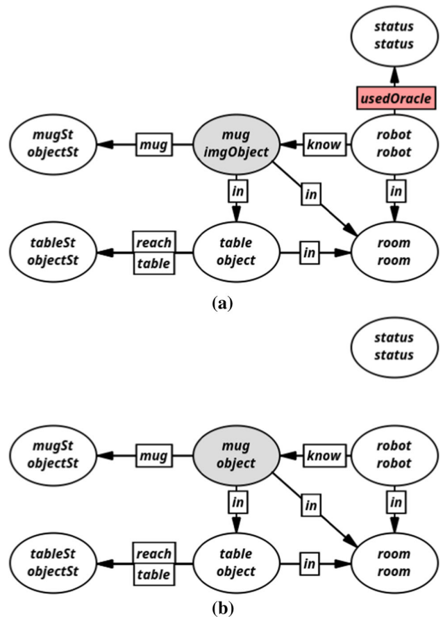
Fig. 7 The action “ verifyImaginaryMug ” describes the preconditions to verify the existence of an imaginary mug (a) and how performing such action affects the internal world model (b). a Action “ verifyImaginaryMug ”: LHS. b Action “ verifyImaginaryMug ”: RHS
