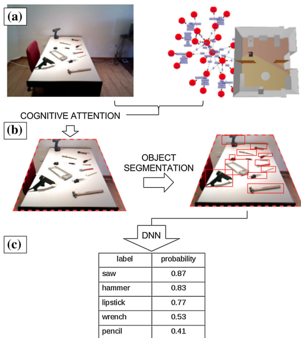
Fig. 9 Pipeline used to extract labels from the camera of the robot: a the geometric model extracted from the semantic network and the robot image is used to extract the region of interest; b then, the object segmentation is fed to the deep neural network; c the result of this process is a list of the possible objects detected in the figure and their associated probability
