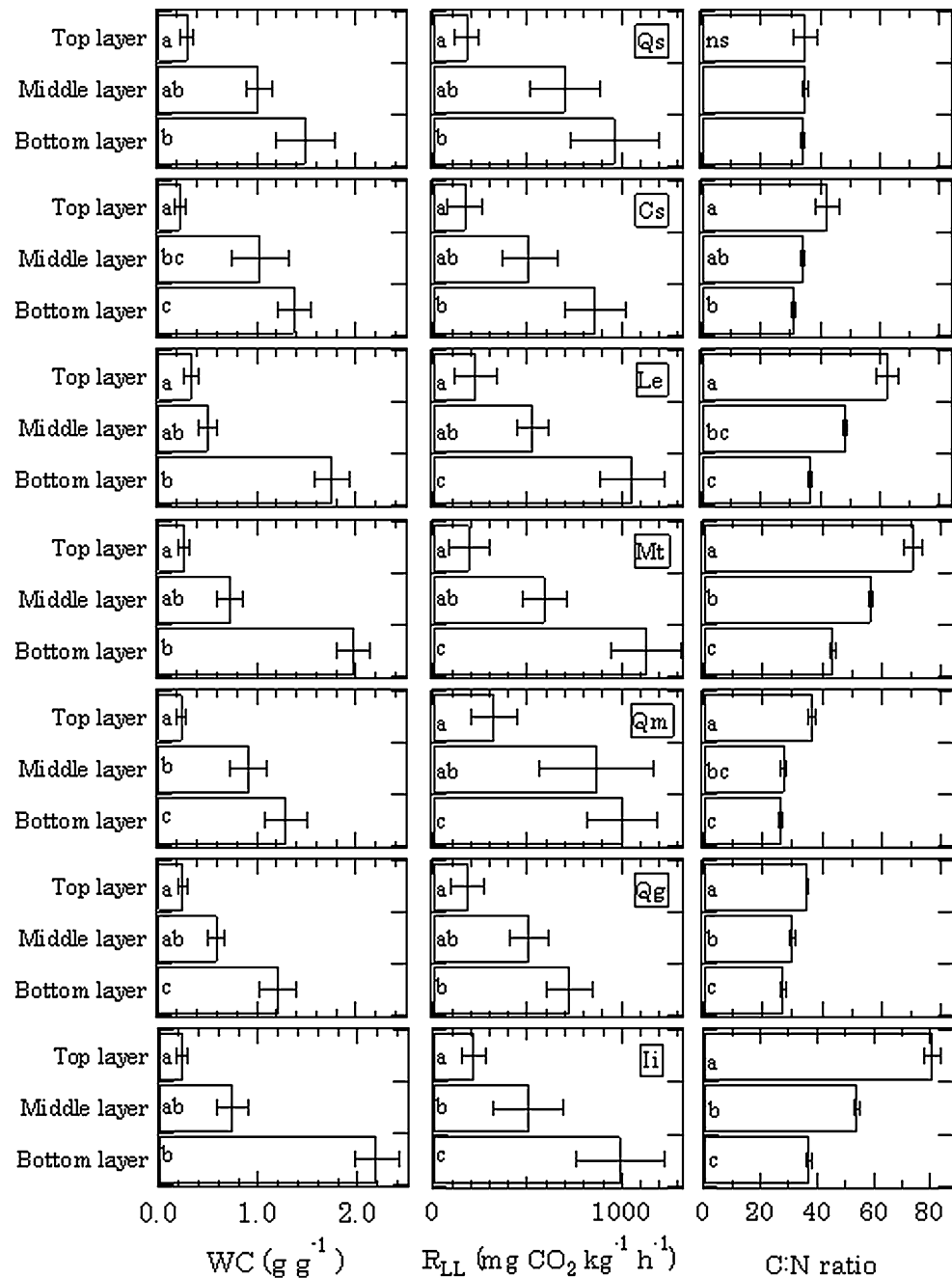
Fig. 2 Vertical spatial variation in the mean R_{LL} , WC , and C:N ratio inside the L layer (top, middle, and bottom layers) among the seven species. Bars indicate standard error. Different letters on the bar indicate significant differences among three layers (Tukey's HSD, P < 0.05 )
