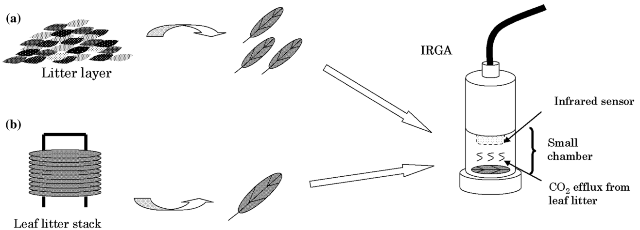
Fig. 1 Illustration of R_{LL} measurements. Measurements of R_{LL} were conducted by sampling leaf litter from (a) seven species and (b) three species. a The L layer was categorized into three layers, and R_{LL} was measured from three leaves in each layer. b A set of 10 dead leaves
