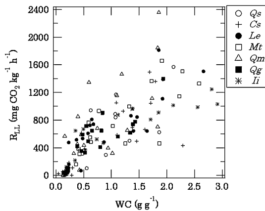
Fig. 3 Relationships between R_{LL} and WC of the seven species
