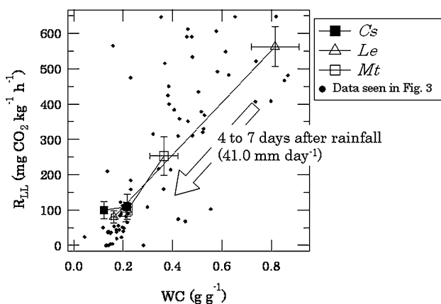
Fig. 4 Temporal variation in mean R_{LL} and WC among three species, 4 to 7 days following rainfall ( 41.0 \text{ mm day}^{-1} ), measured in August 2010. Mean R_{LL} and WC were calculated from 10 dead leaves composing one leaf litter stack (Fig. 1b). Bars indicate standard error. Closed circles indicate the relationships between R_{LL} and WC as seen in Fig. 3
