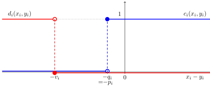
Fig. 2 Shapes of the single criterion concordance index c_i(x_i, y_i) and the discordance index d_i(x_i, y_i) in the style of ELECTRE I. Empty (resp. filled) circles indicate excluded (resp. included) values
