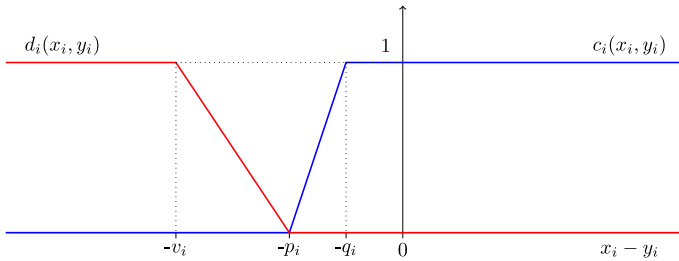
Fig. 1 Shapes of the single criterion concordance index c_i(x_i, y_i) and the discordance index d_i(x_i, y_i) in ELECTRE III and ELECTRE TRI
