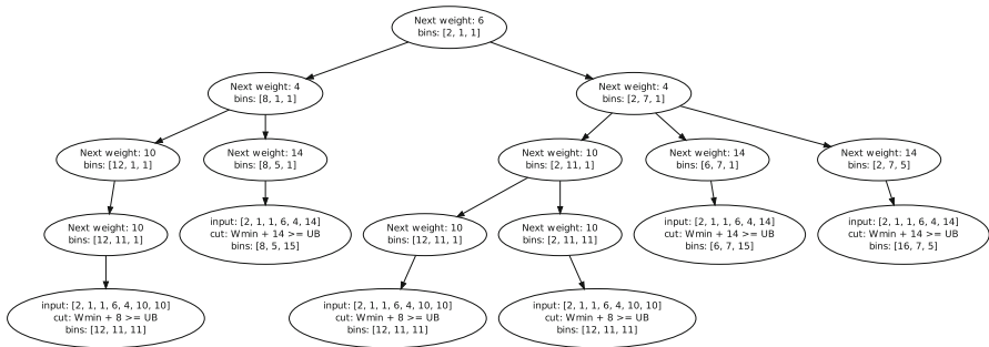
Fig. 11 Subtree 11, layout [2, 1, 1], items (2,1,1)
