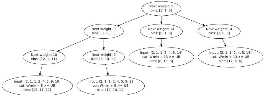
Fig. 10 Subtree 8, layout [3, 1, 6], items (2,1,1,2,4)
