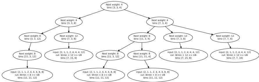
Fig. 7 Subtree 5, layout [3, 3, 4], items (2,1,1,2,4)
