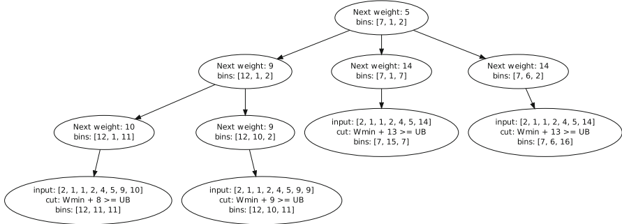
Fig. 9 Subtree 7, layout [7, 1, 2], items (2,1,1,2,4)
