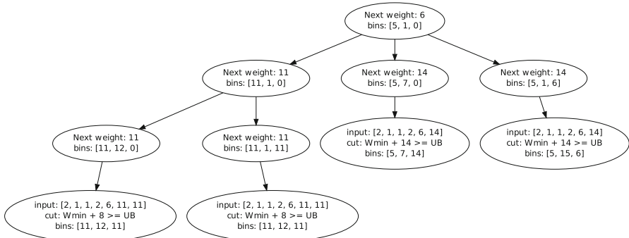
Fig. 8 Subtree 6, layout [5, 1, 0], items (2,1,1,2)
