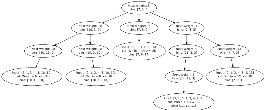
Fig. 4 Subtree 2, layout [7, 3, 0], items (2,1,3,4)
