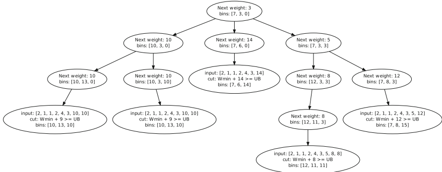
Fig. 6 Subtree 4, layout [7, 3, 0], items (2,1,1,2,4)
