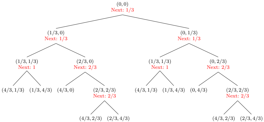
Fig. 1 4/3 lower bound decision tree. Player 1 decisions are the “Next: w_i ”. The pairs (w_1, w_2) are corresponding to the space used in the bins
