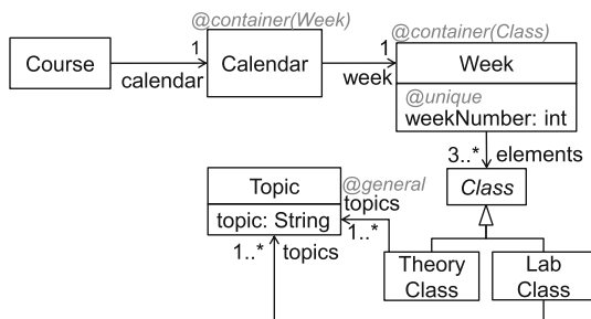
Fig. 9 Meta-model induced from the fragment in Listing 3
