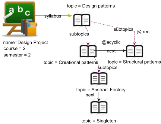
Fig. 16 Fragment describing the structure of the syllabus
